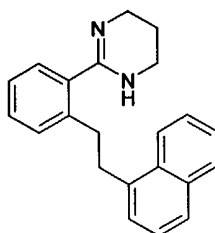
Compound HO
