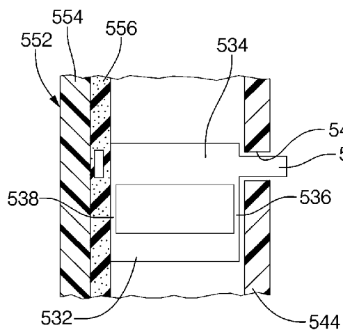
PRIOR ART FIG. 44
