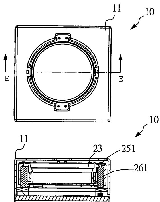
E-E Section
