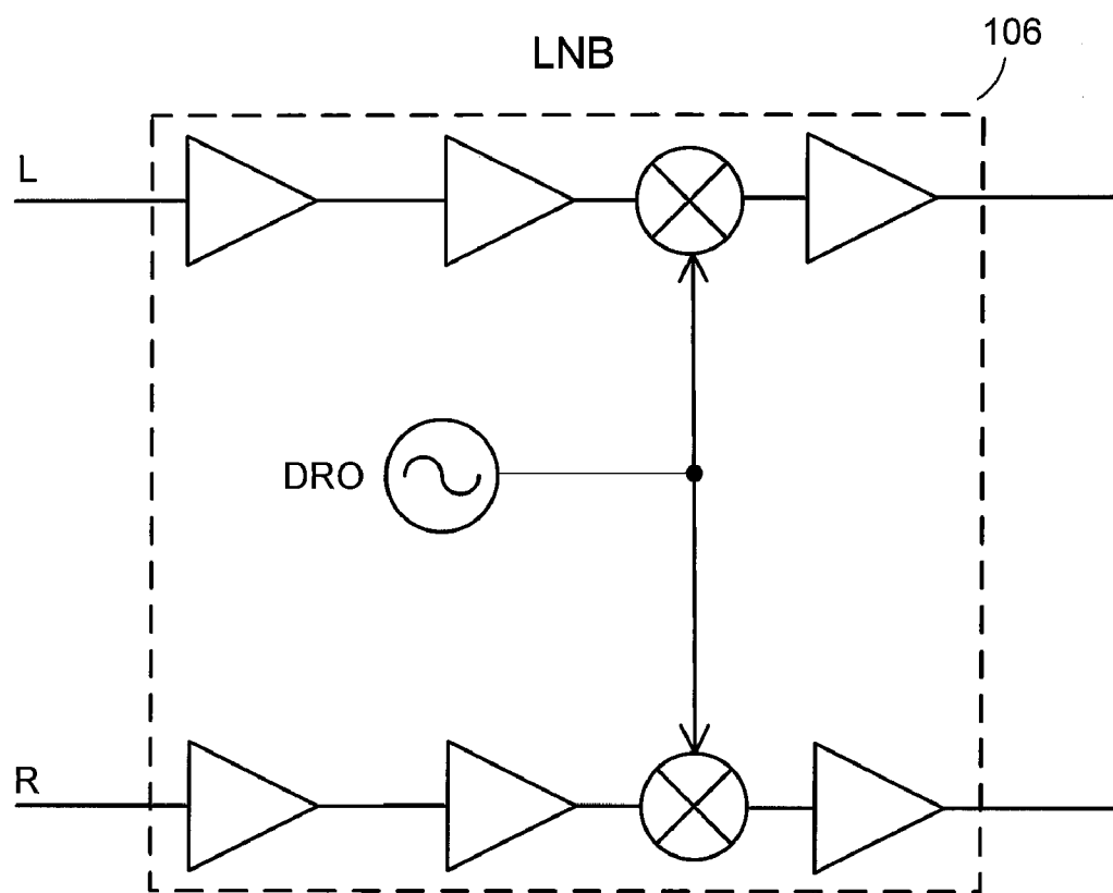
Example of LNB with DRO LO
