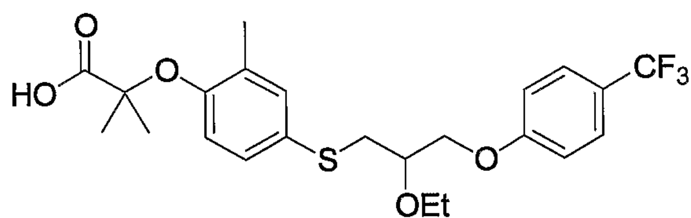
2-{4-[2-Ethoxy-3-(4-trifluoromethyl-phenoxy)-propylsulfanyl]-2-methyl-phenoxy}-2-methyl-propionic acid
