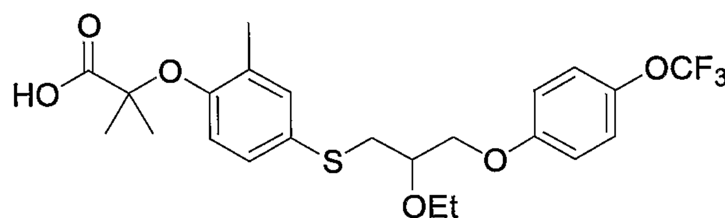
Compound 9
