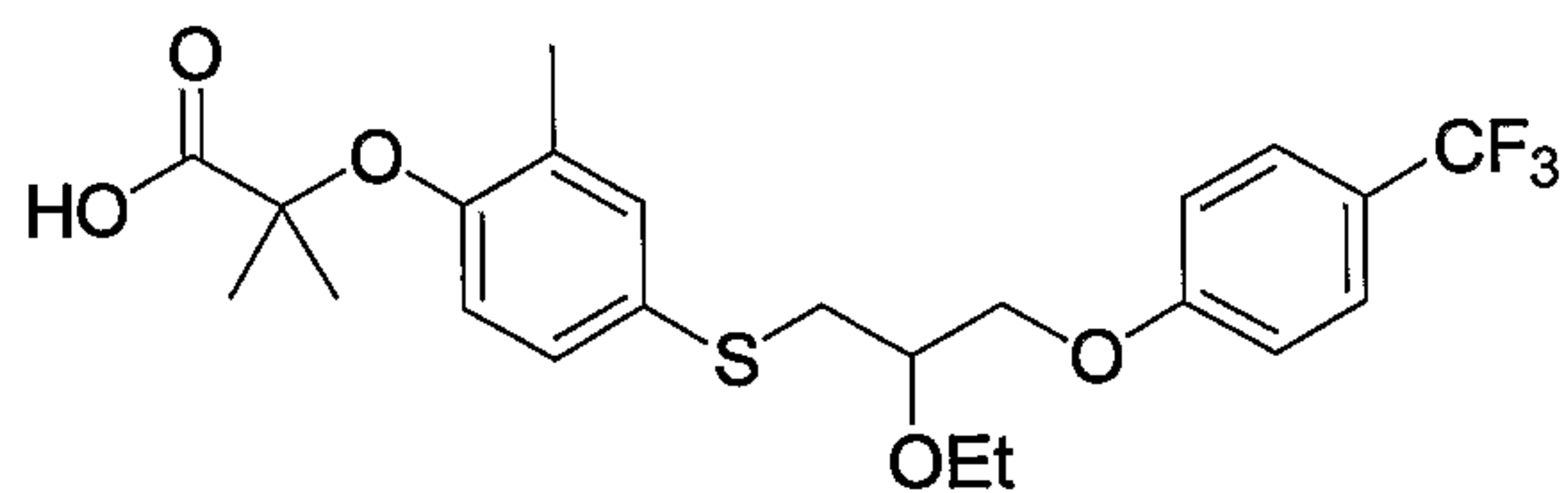
Compound 3
