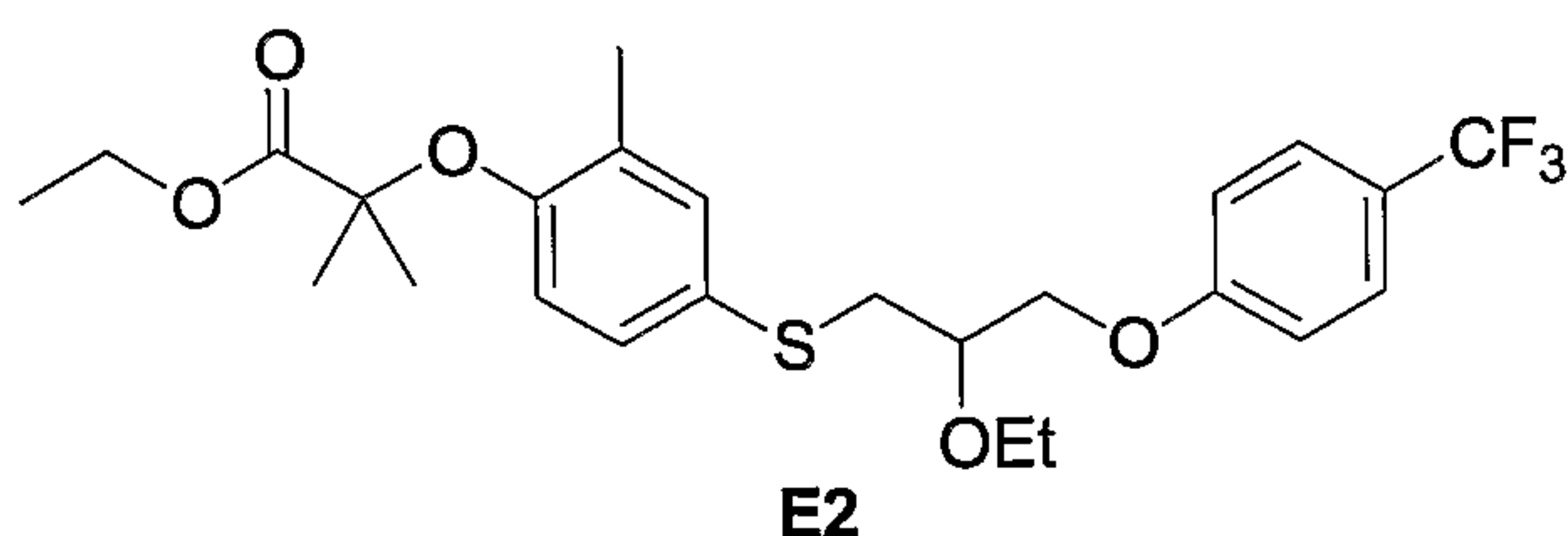
2-{4-[2-Ethoxy-3-(4-trifluoromethyl-phenoxy)-propylsulfanyl]-2-methyl-phenoxy}-2-methyl-propionic acid ethyl ester
