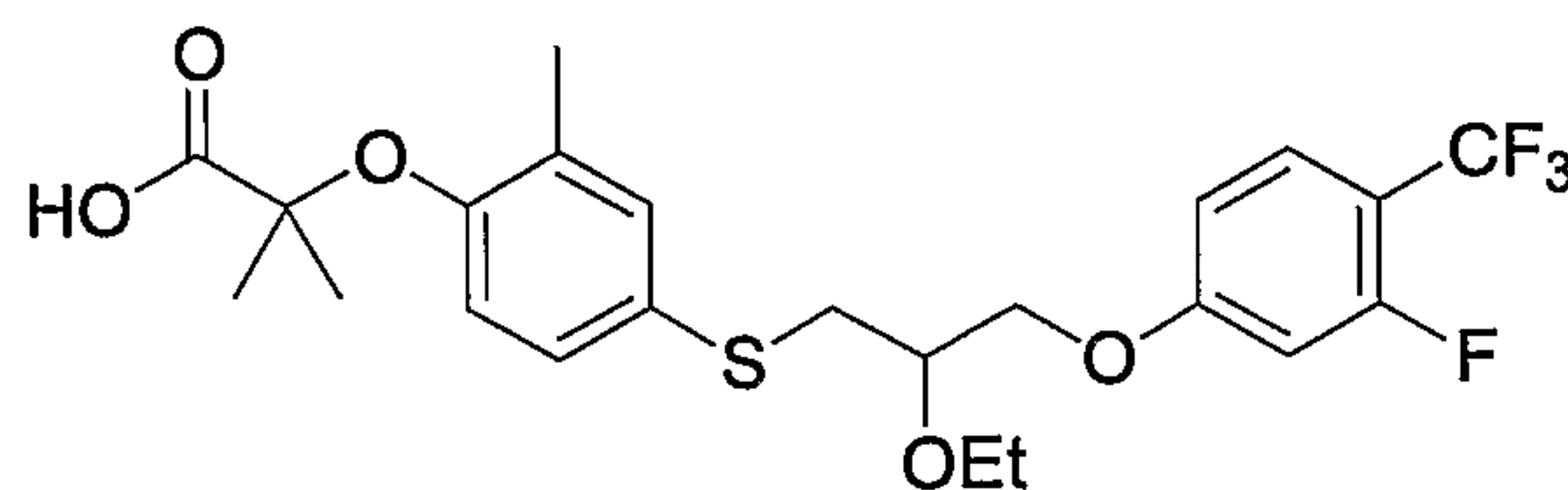
Compound 12
