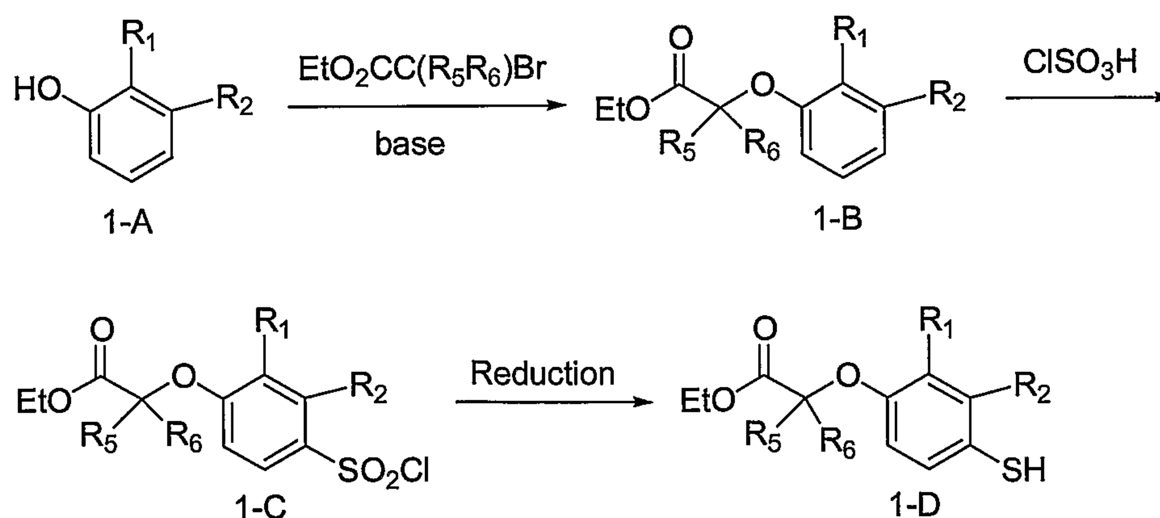
Scheme 1. Synthesis of Intermediate 1-D
