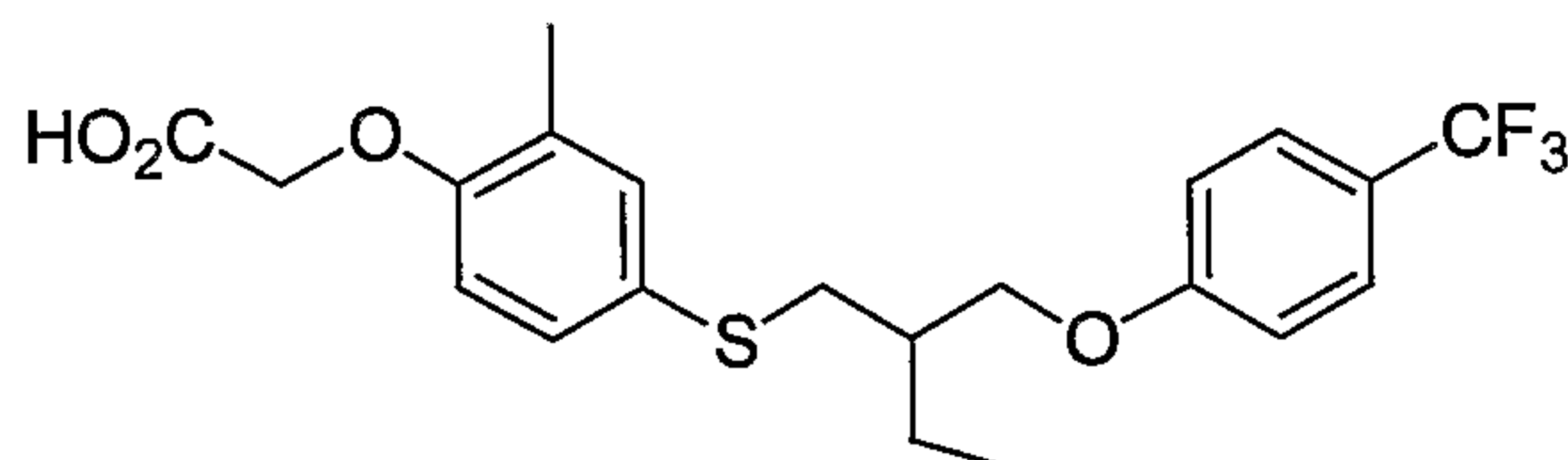
{2-Methyl-4-[2-(4-trifluoromethyl-phenoxy)methyl]-butylsulfanyl}-phenoxy}-acetic acid
