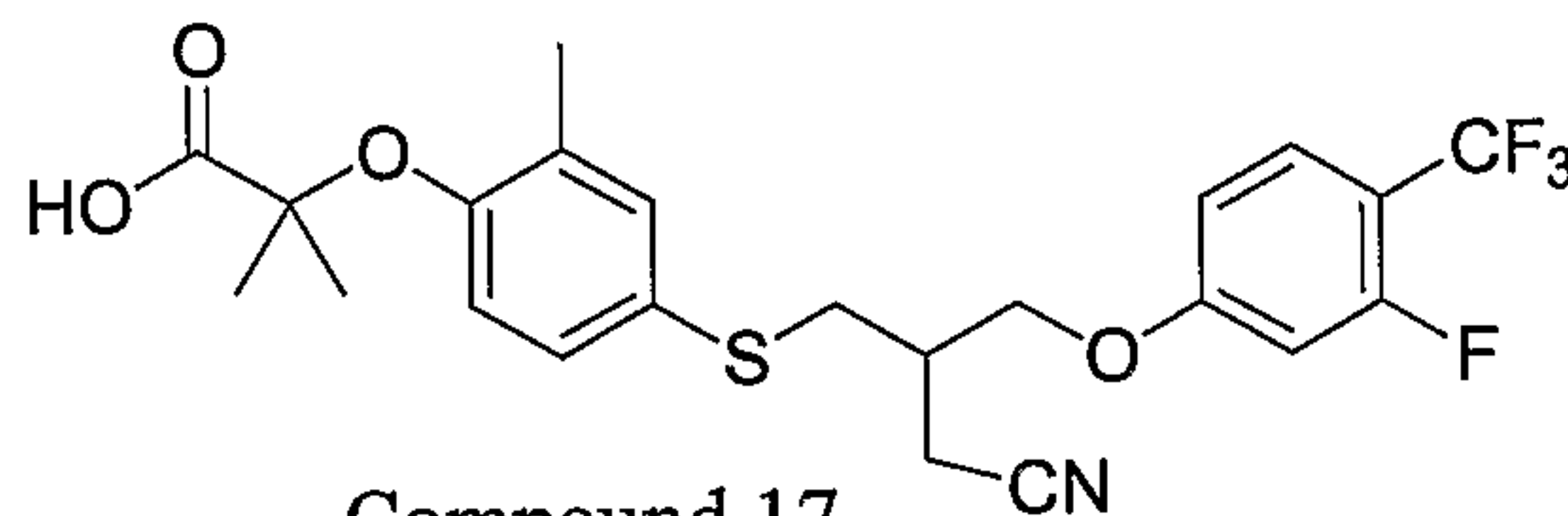
Compound 17
