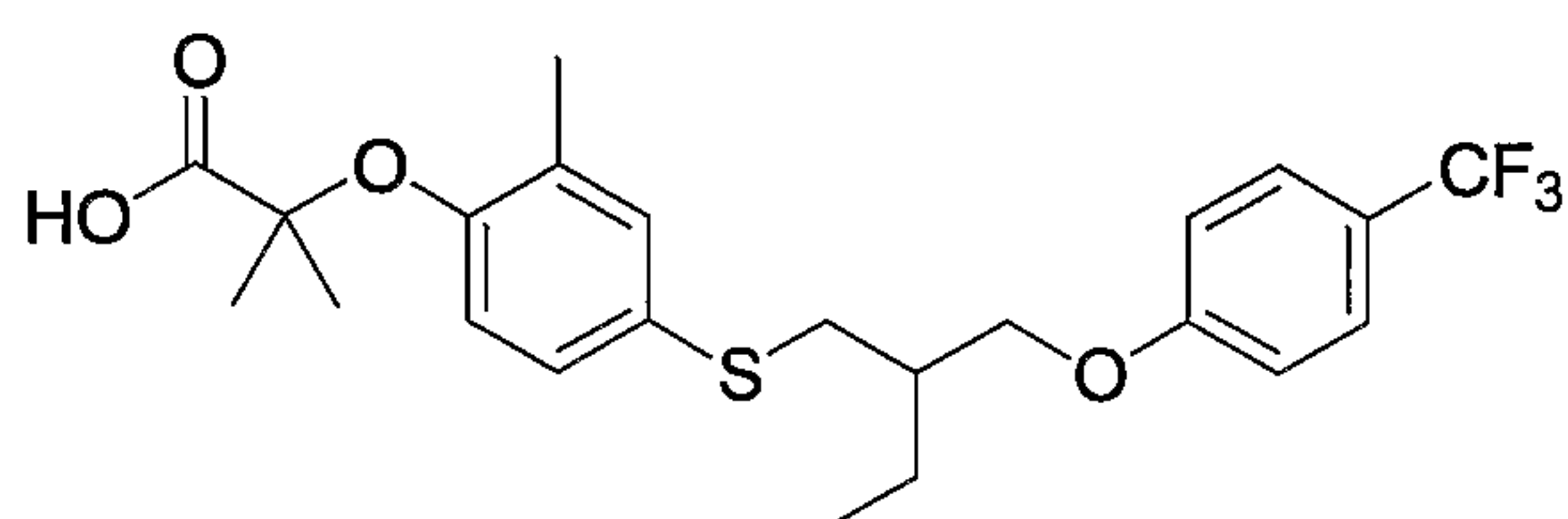
Compound 2
