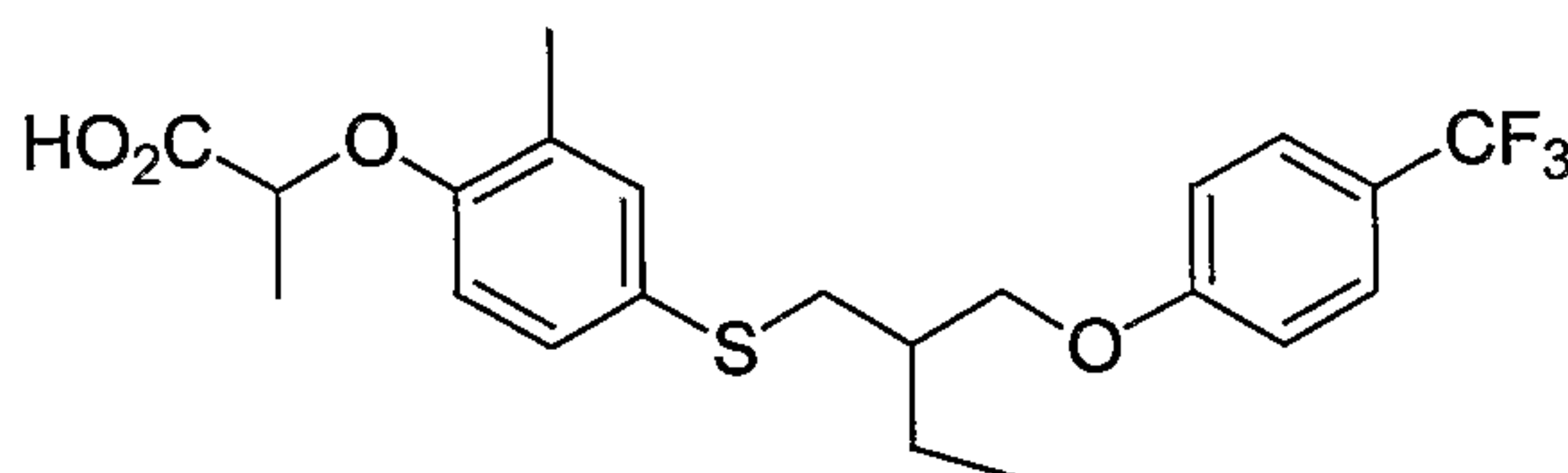
Compound 1
