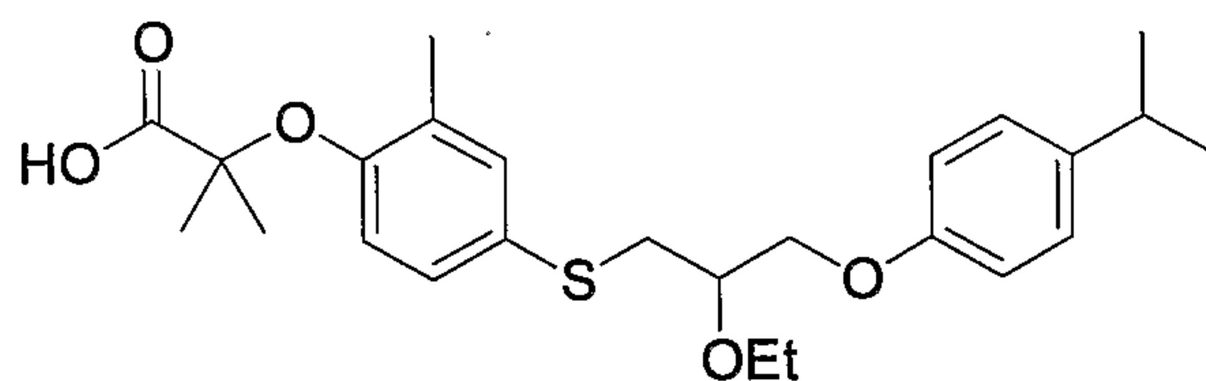
Compound 8
