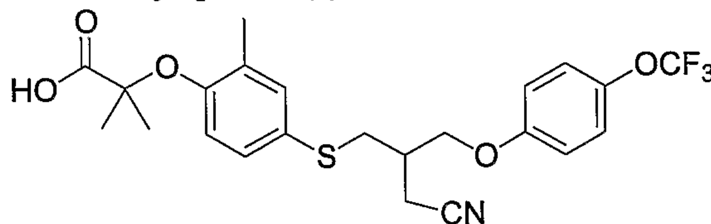
Compound 14
