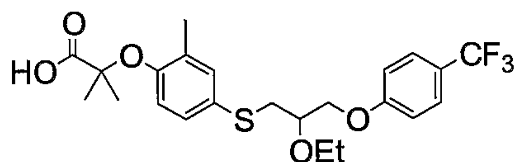
Compound 3
