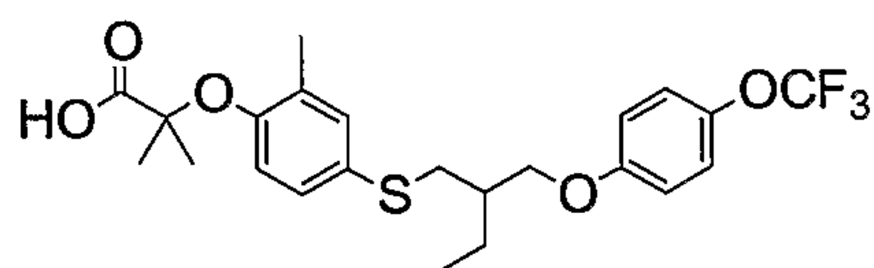
Compound 4
