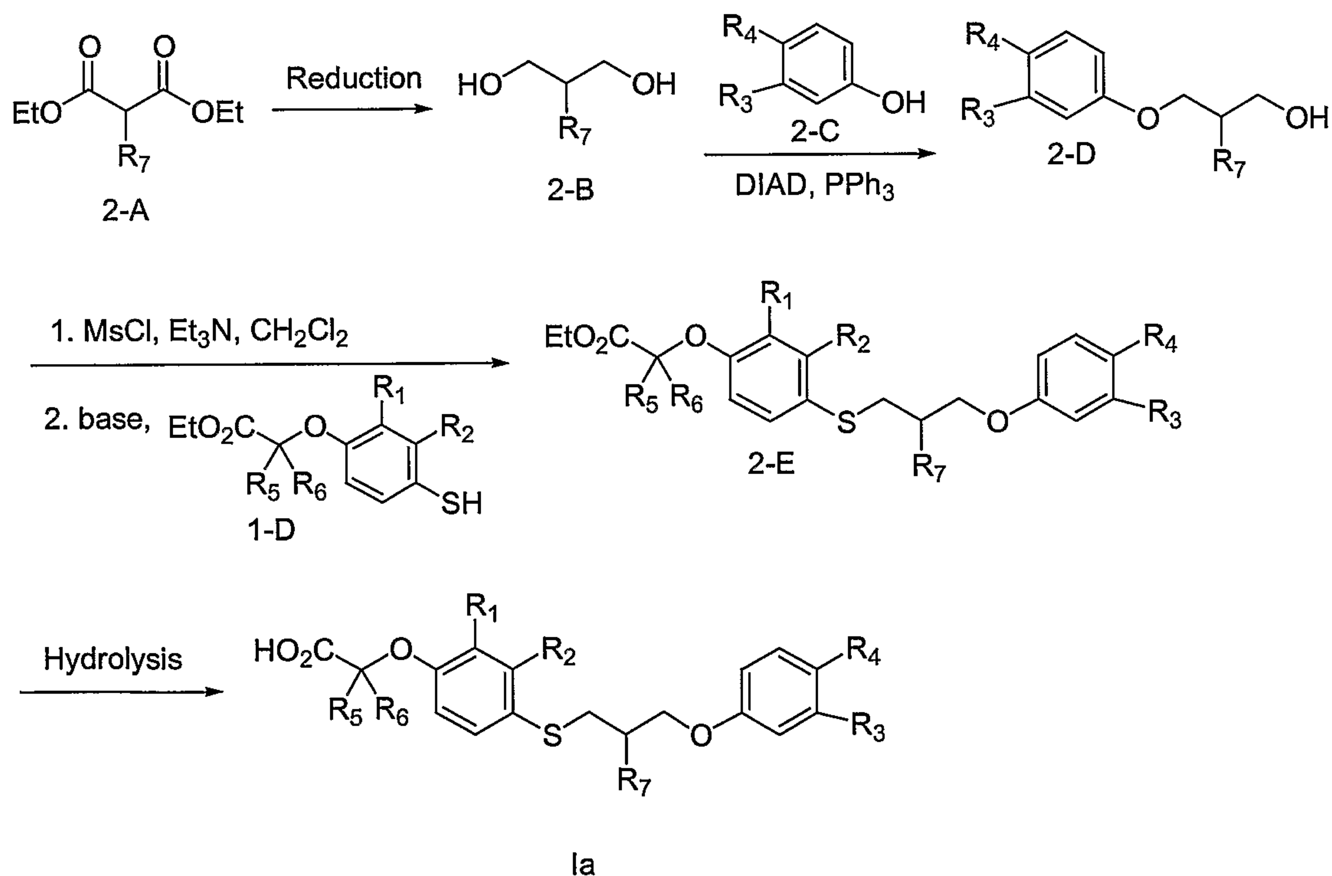
Scheme 2. Synthesis of Compound Ia
