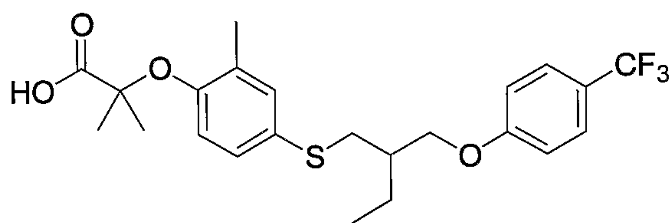
compound 4 #26171158#
