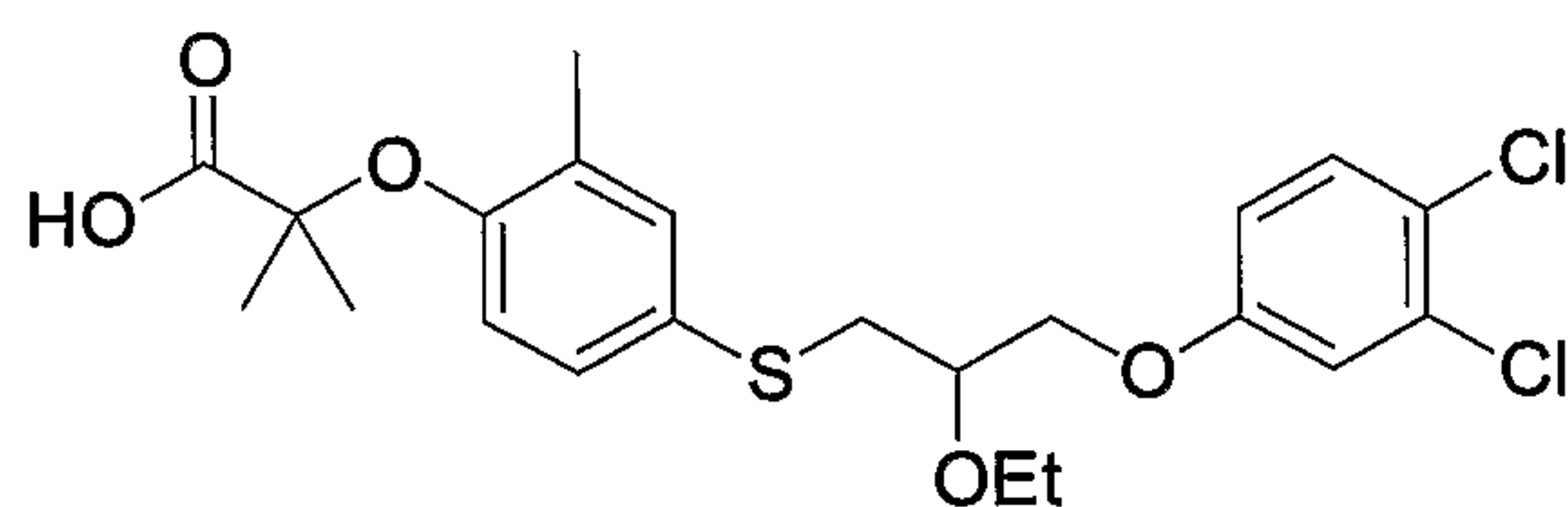
Compound 11
