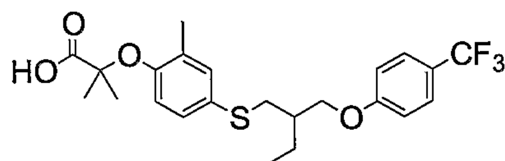
Compound 1
