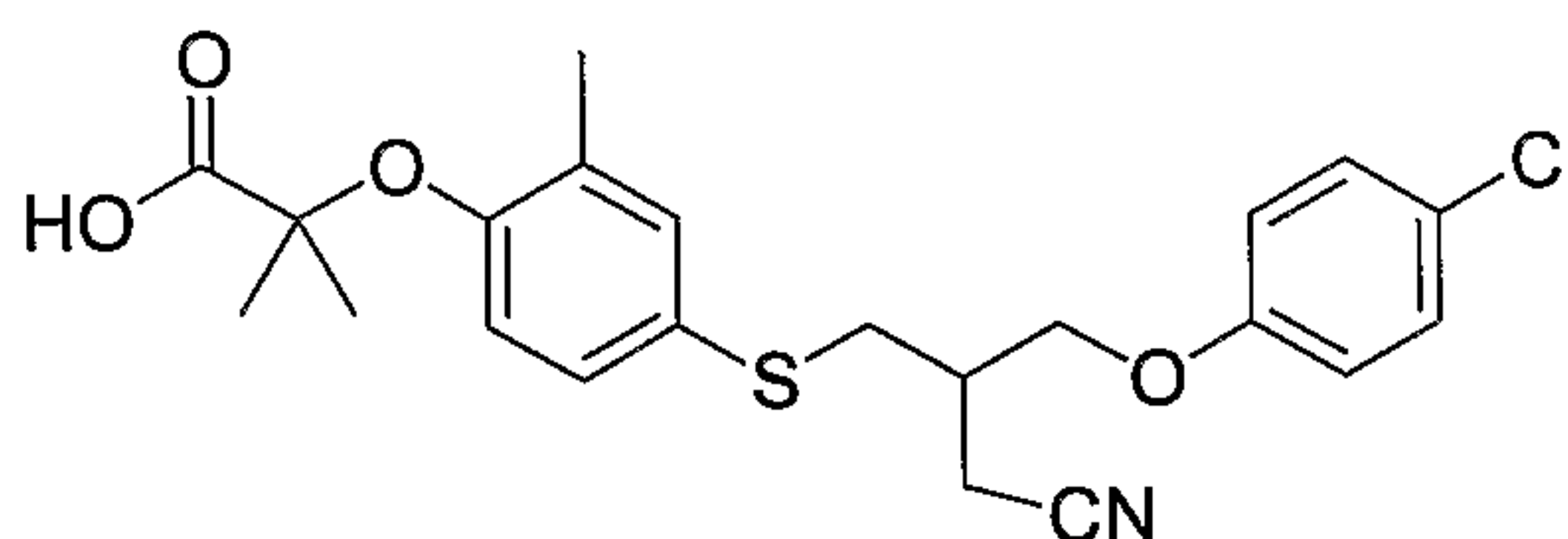
Compound 15
