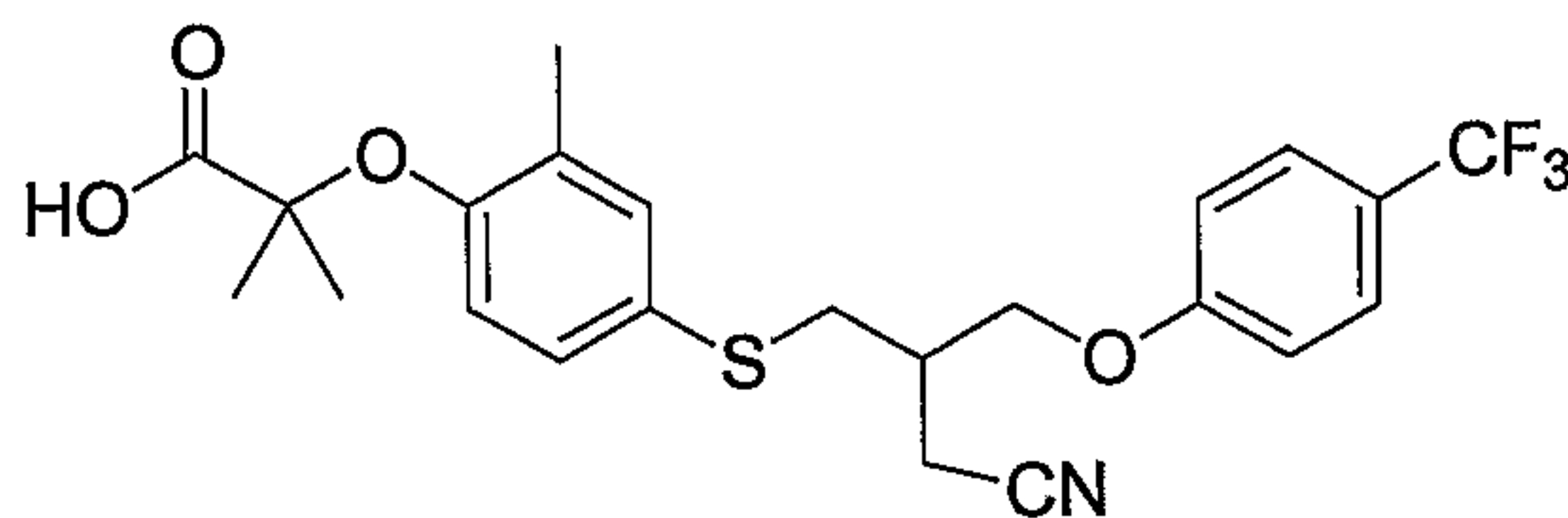
Compound 18
