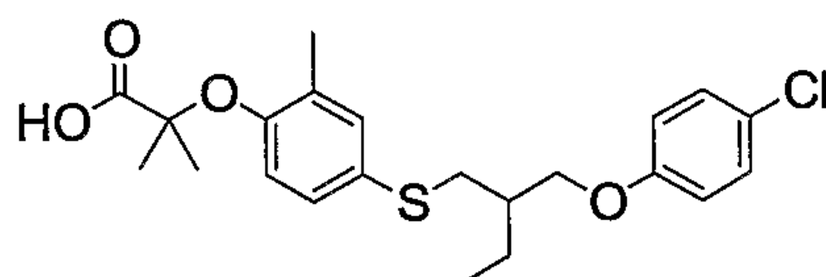
Compound 5
