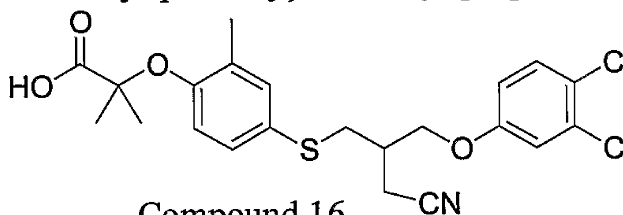
Compound 16
