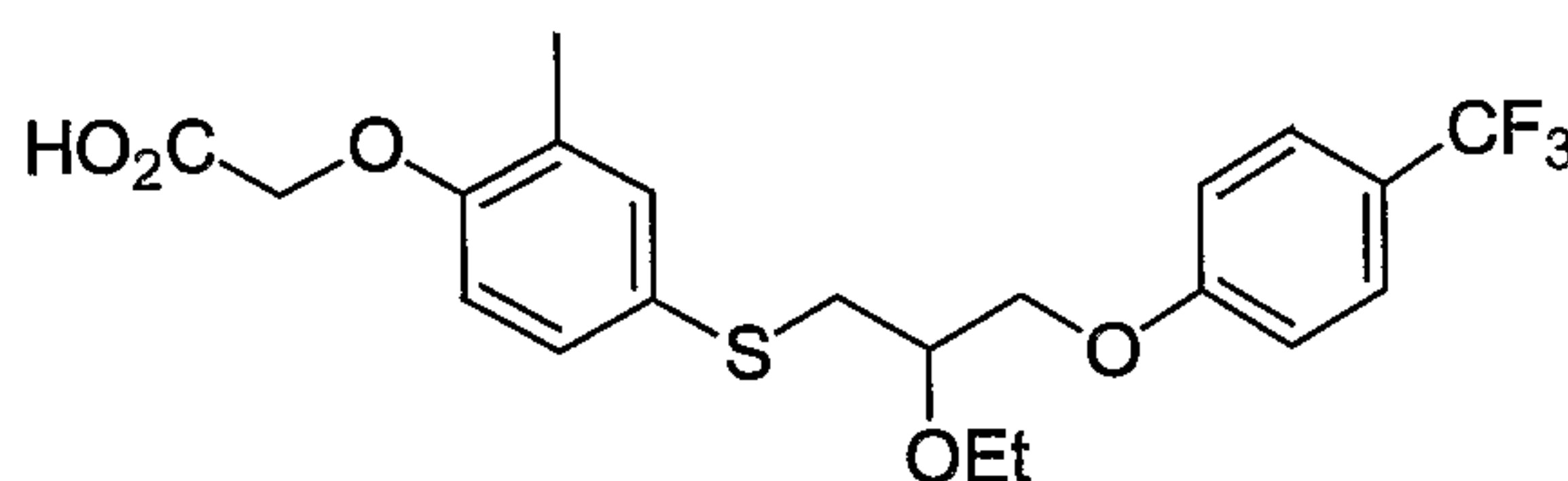
{4-[2-Ethoxy-3-(4-trifluoromethyl-phenoxy)-propylsulfanyl]-2-methyl-phenoxy}-acetic acid
