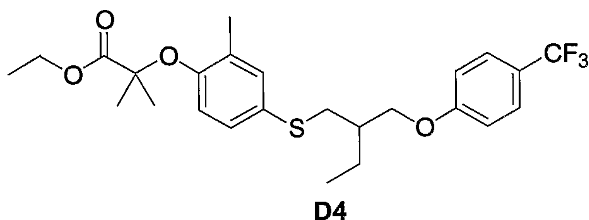
2-Methyl-2-{2-methyl-4-[2-(4-trifluoromethyl-phenoxy)methyl]-butylsulfanyl]-phenoxy}-propionic acid ethyl ester
