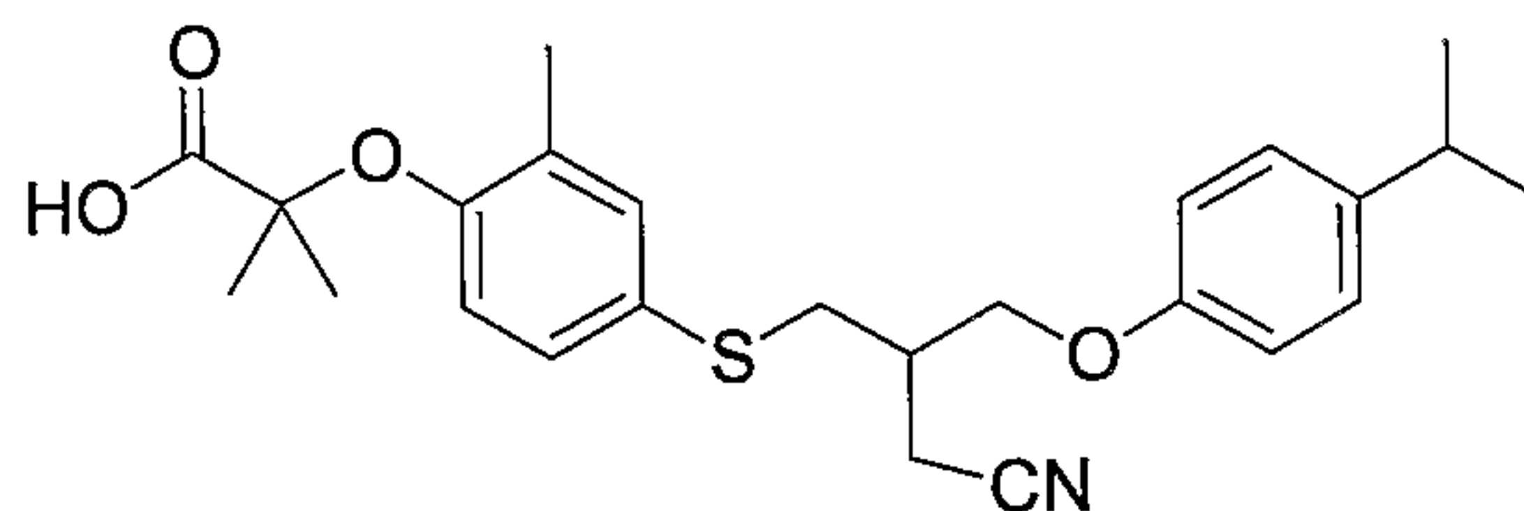
Compound 13
