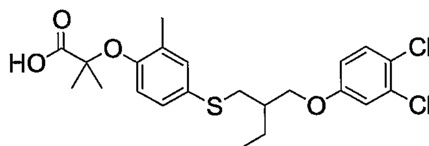
Compound 6
