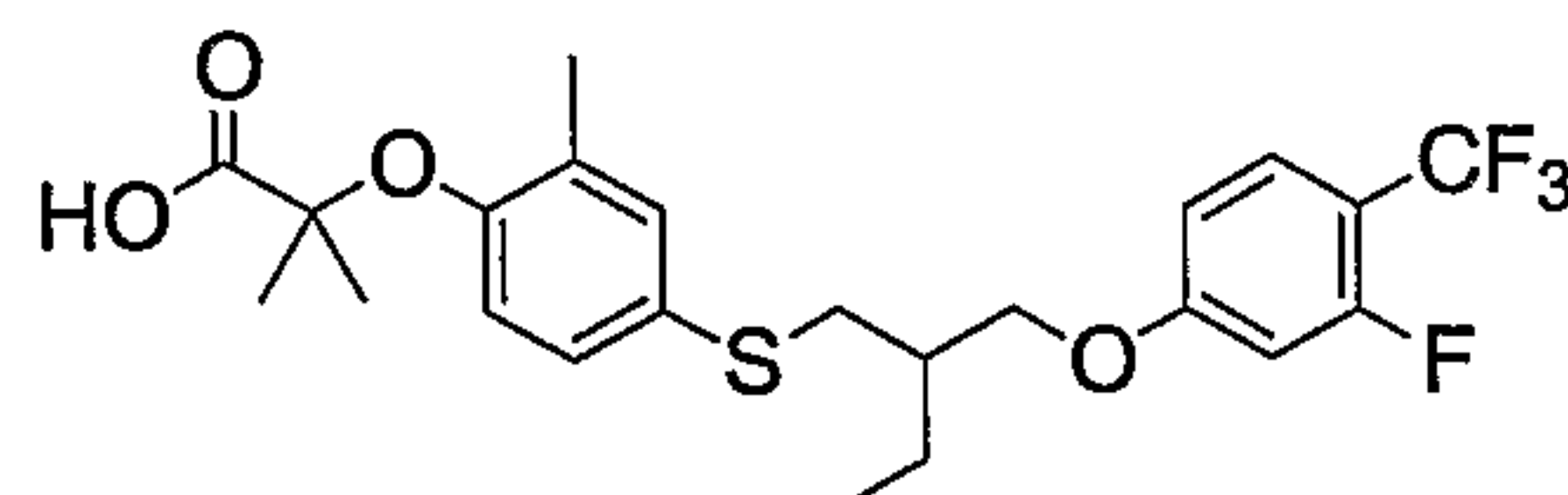
Compound 7
