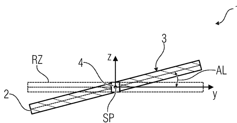
Fig. 2 (PRIOR ART)
