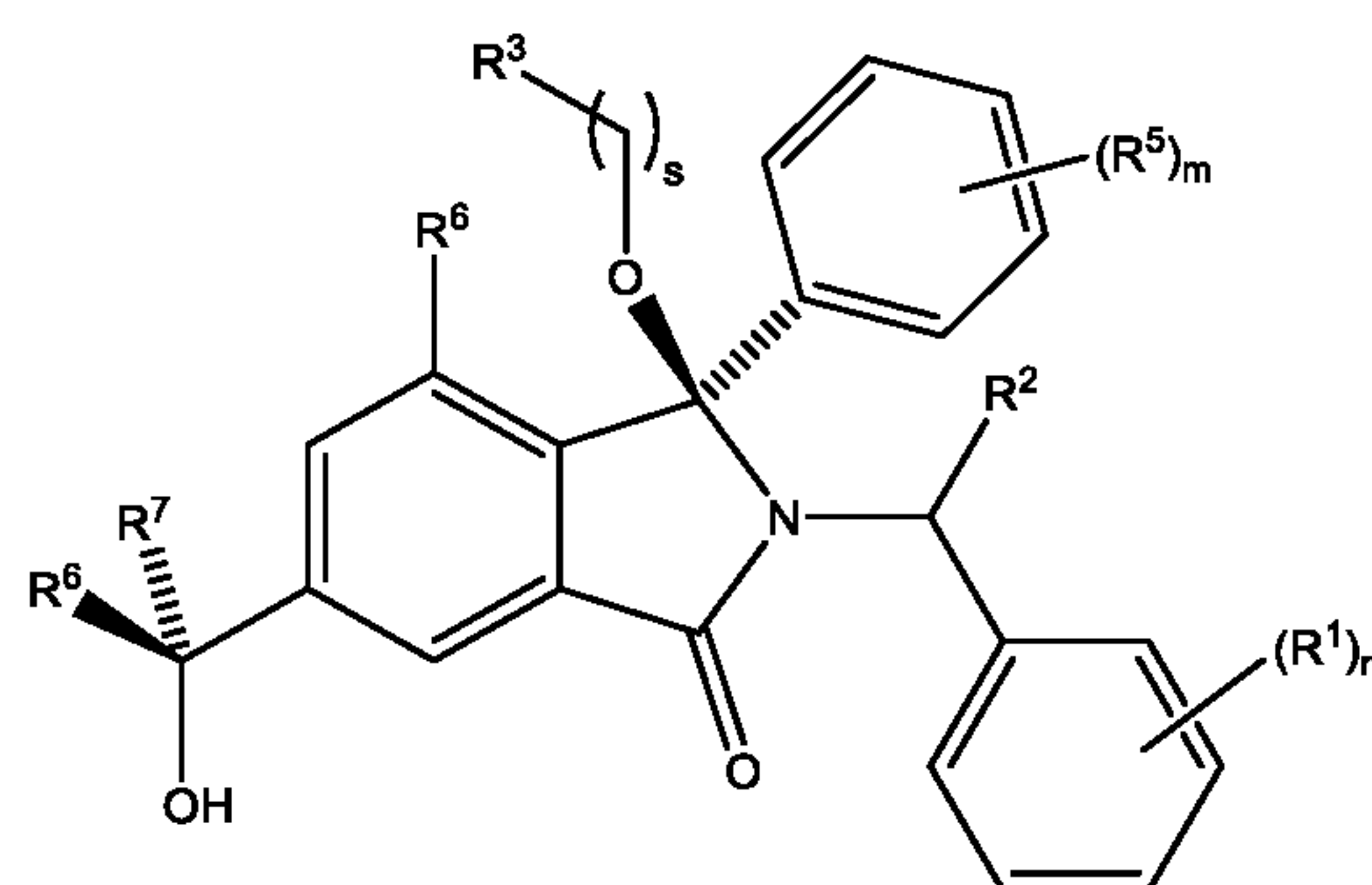
Diastereoisomer 2B
