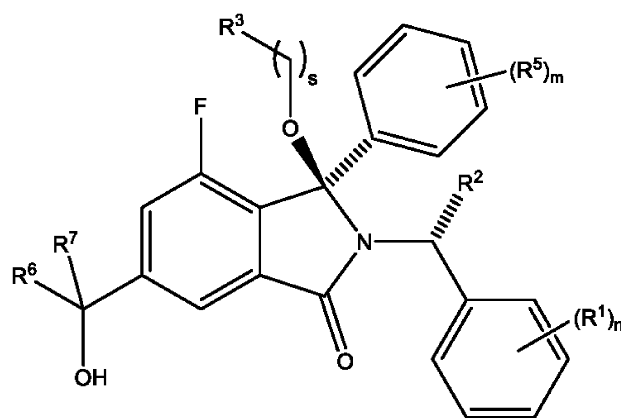
Diastereoisomer 1B
