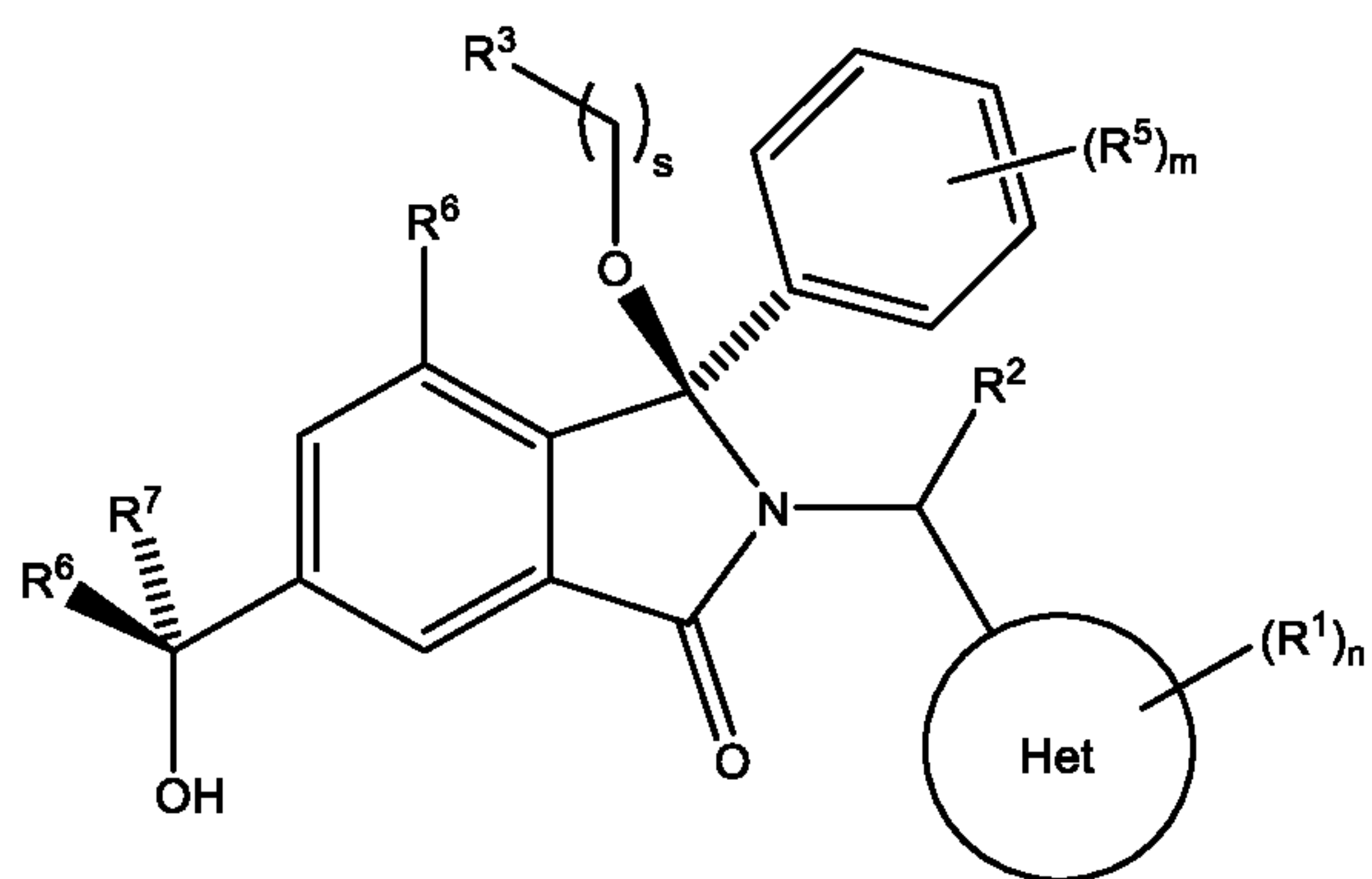
Diastereoisomer 2B
