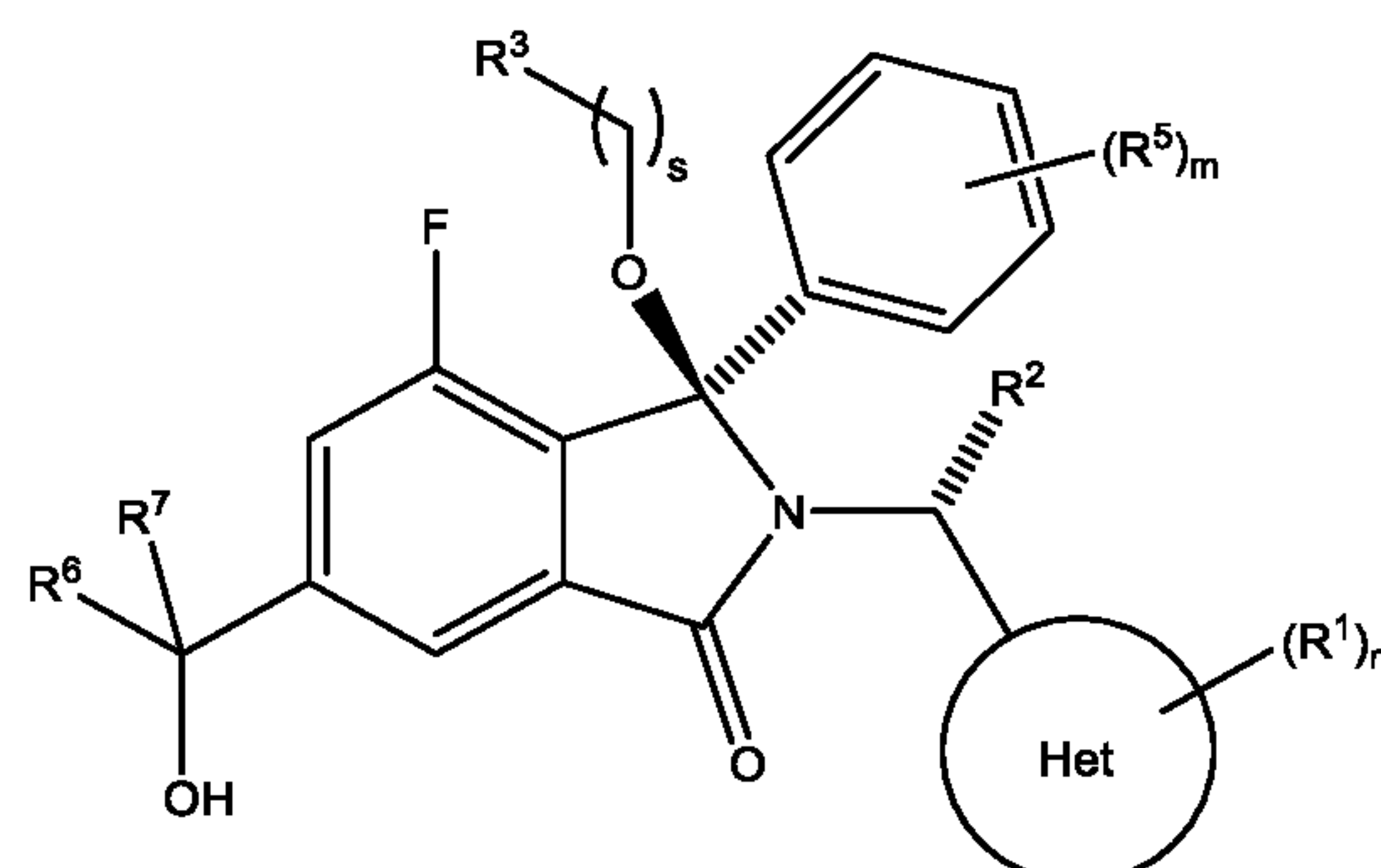
Diastereoisomer 1B
