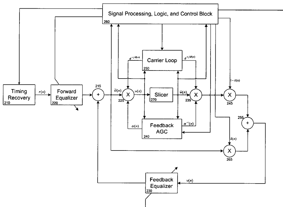
Block diagram of timing recovery, equalization, carrier recovery, and automatic gain control, jointly controlled by a central signal processing block in accordance with the present invention.
