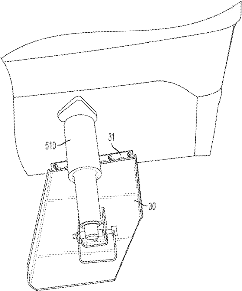
FIG. 2 PRIOR ART
