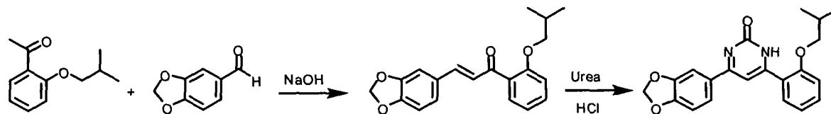
Scheme 4
