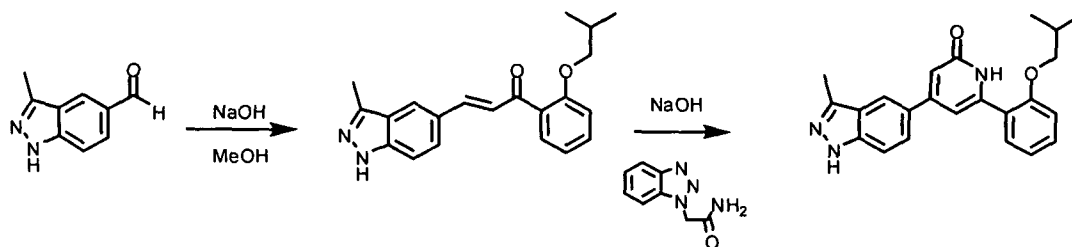
Scheme 7.
