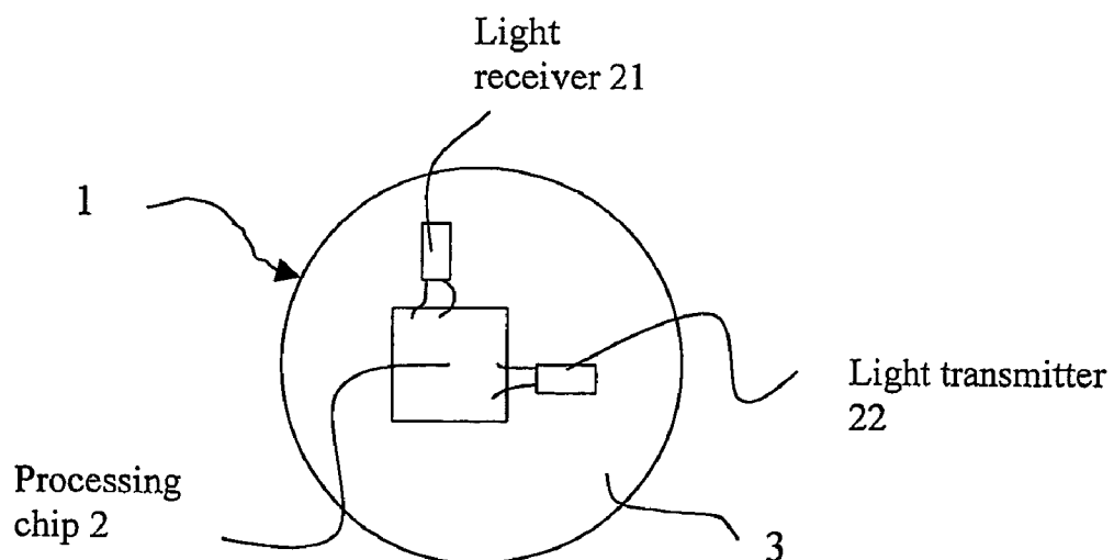
Fig. 2. Diagram of a ball containing processor and optical communication.
