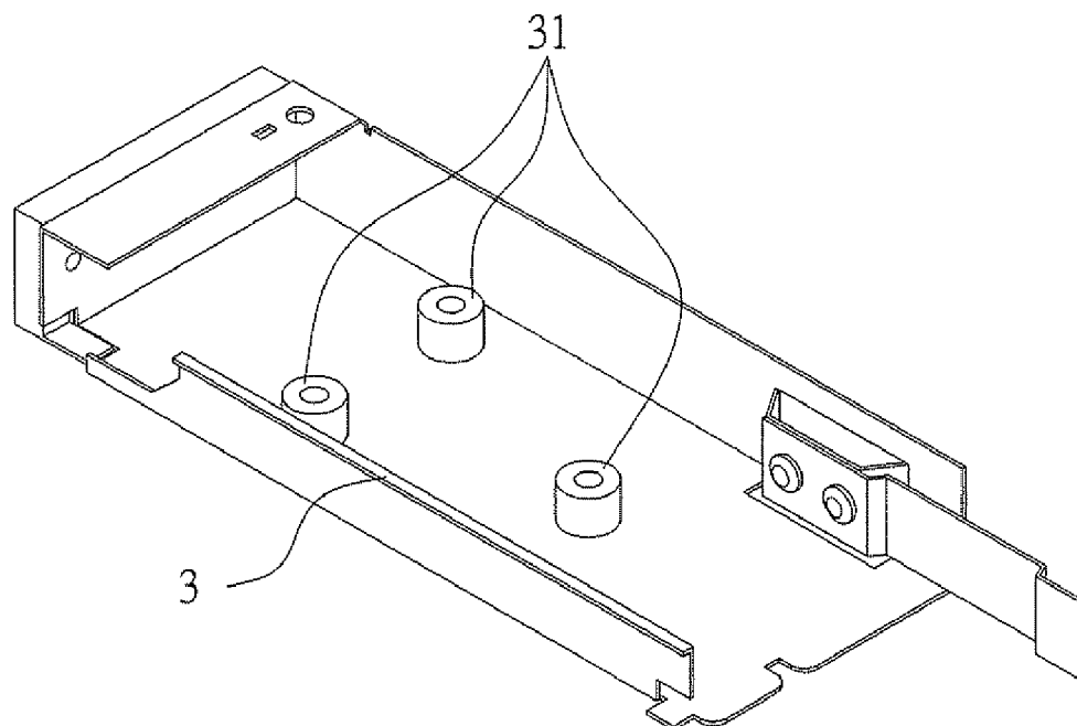
FIG. 4 (PRIOR ART)
