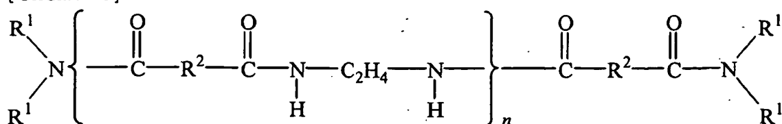
[Chem. 4]
