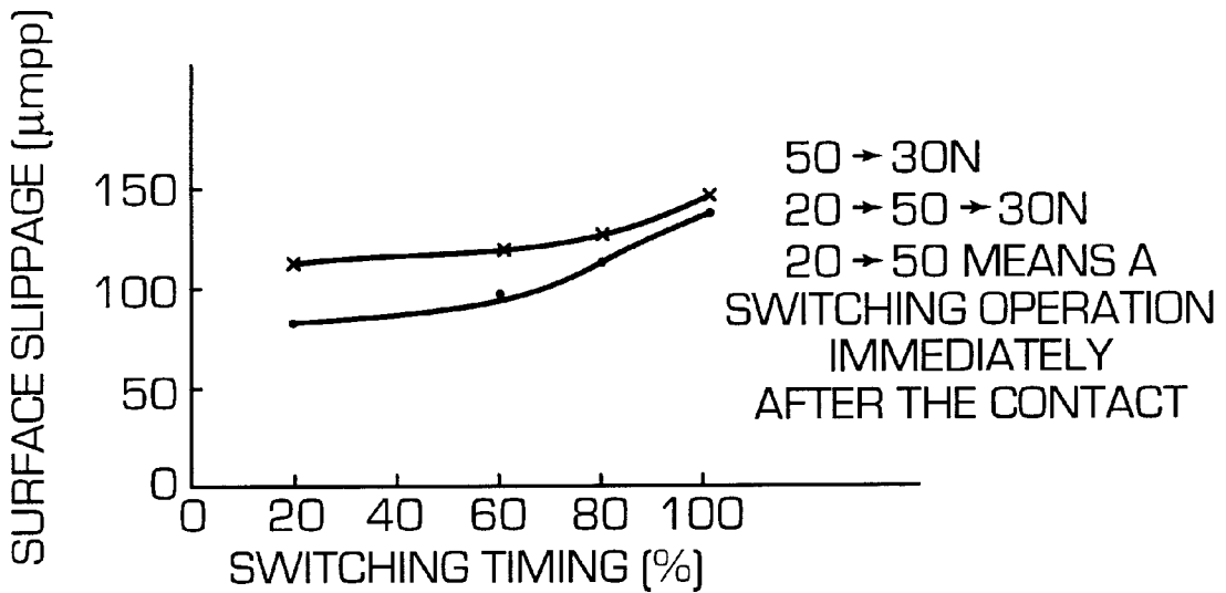
RELATION BETWEEN SURFACE SLIPPAGE AND SWITCHING TIMING
