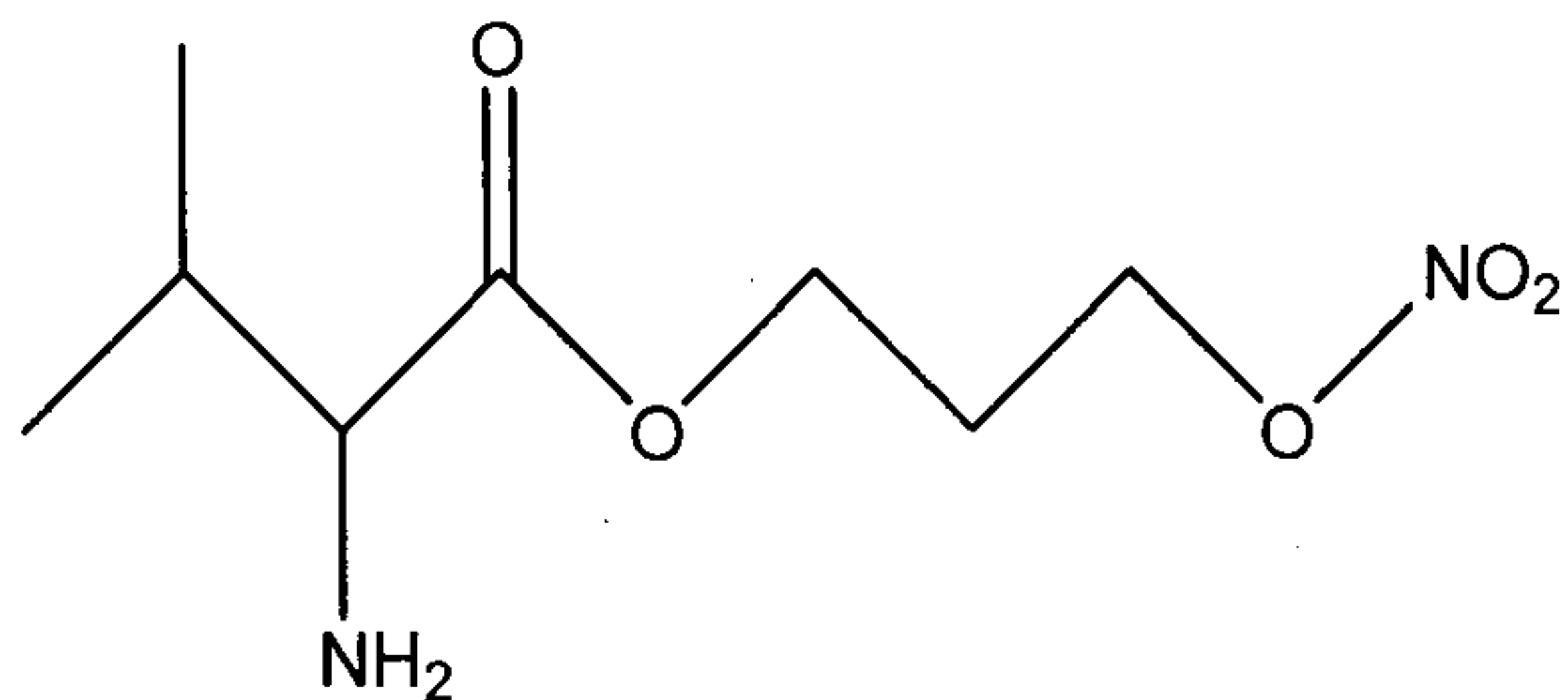
2'-nitrooxypropyl 2-amino-3-methylbutanoate.
