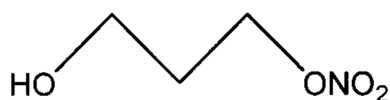
nitrooxyethyl alcohol
