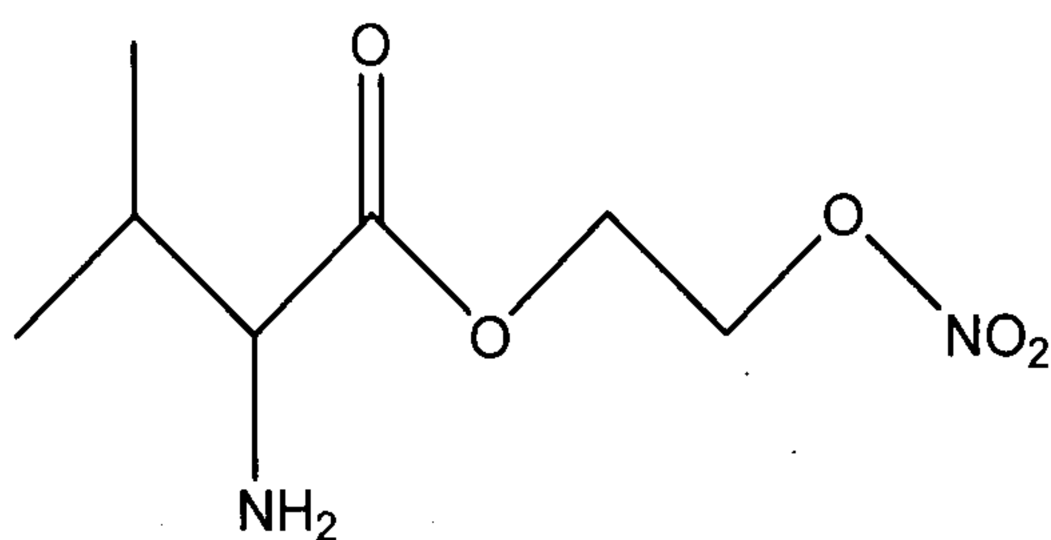
2'-nitrooxyethyl 2-amino-3-methylbutanoate.
