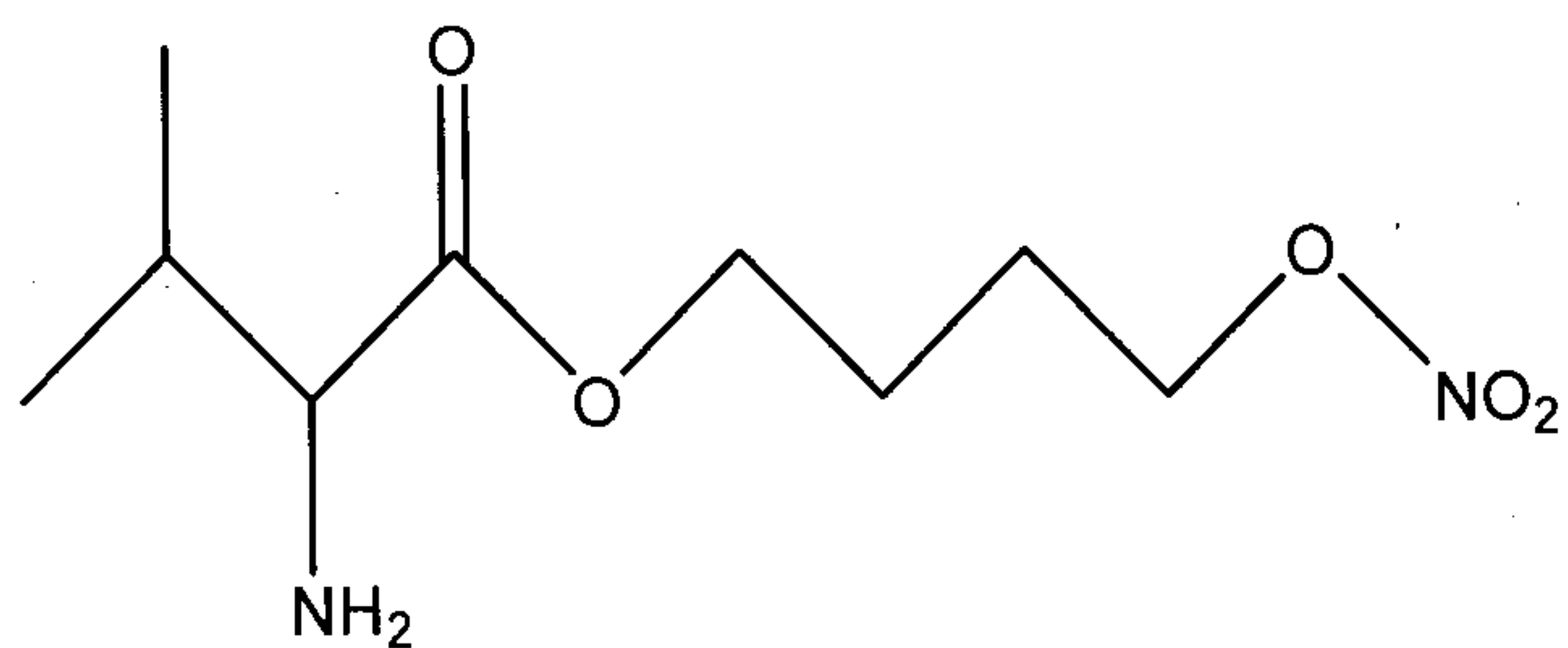
2'-nitrooxybutyl 2-amino-3-methylbutanoate.
