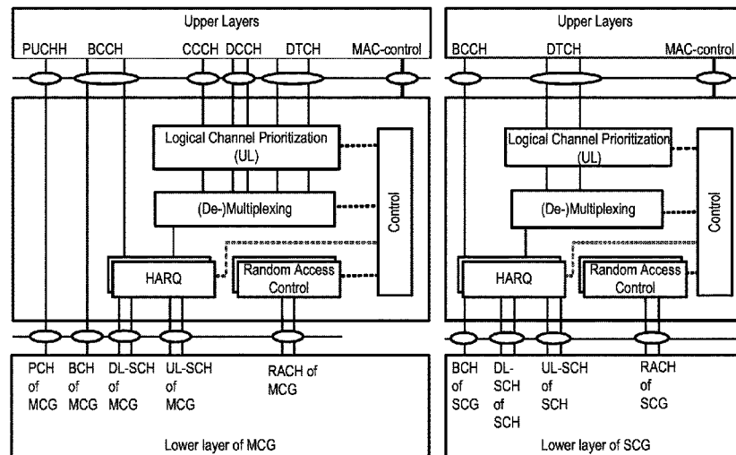
Dual-Connectivity- two MAC entities at UE side
