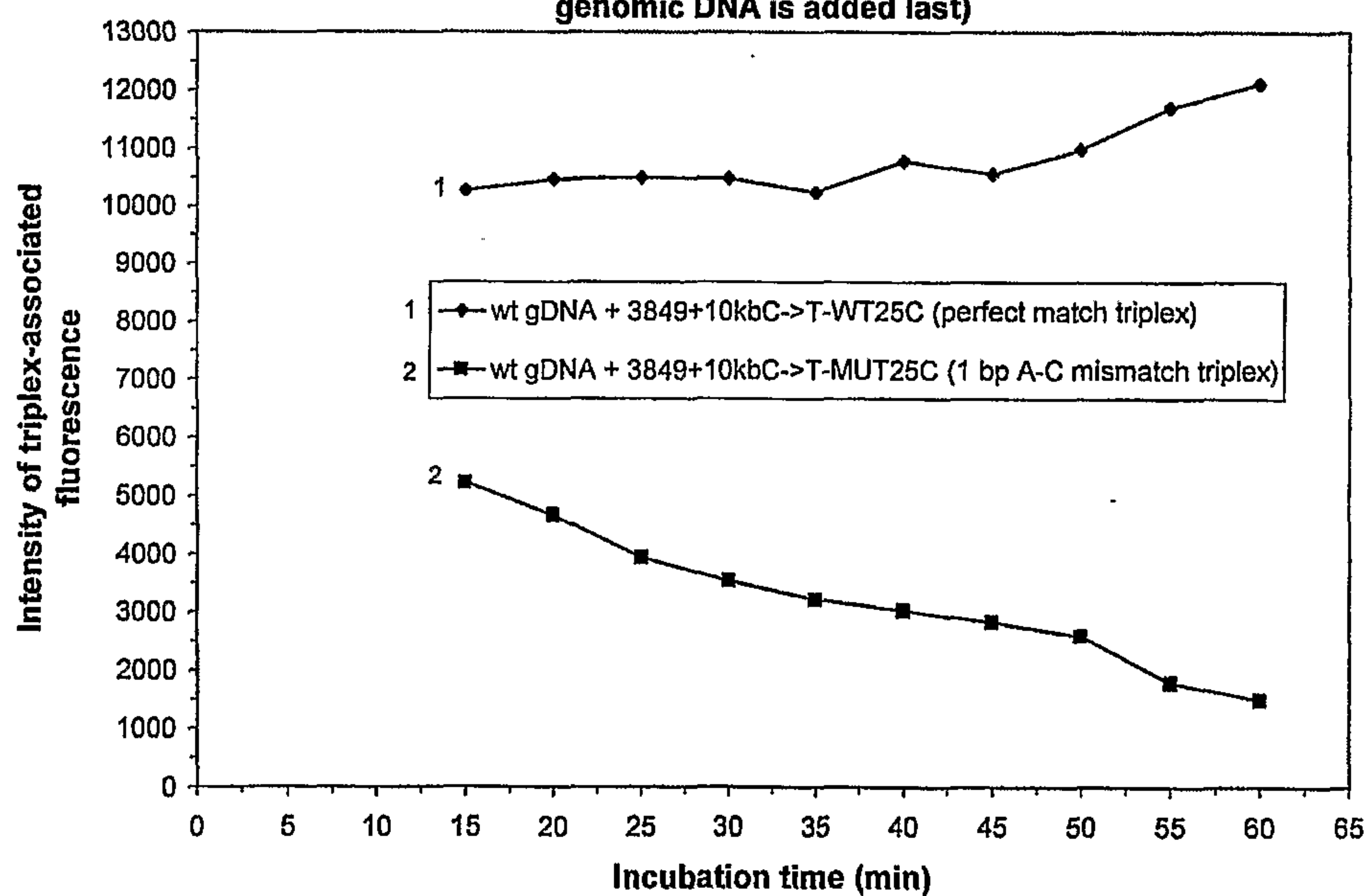
FIG. 4. Triplex-associated fluorescence from human genomic DNA samples assayed in the presence of 500 nM YOYO-1 and 40 mM TMA-Cl (wherein genomic DNA is added last)
