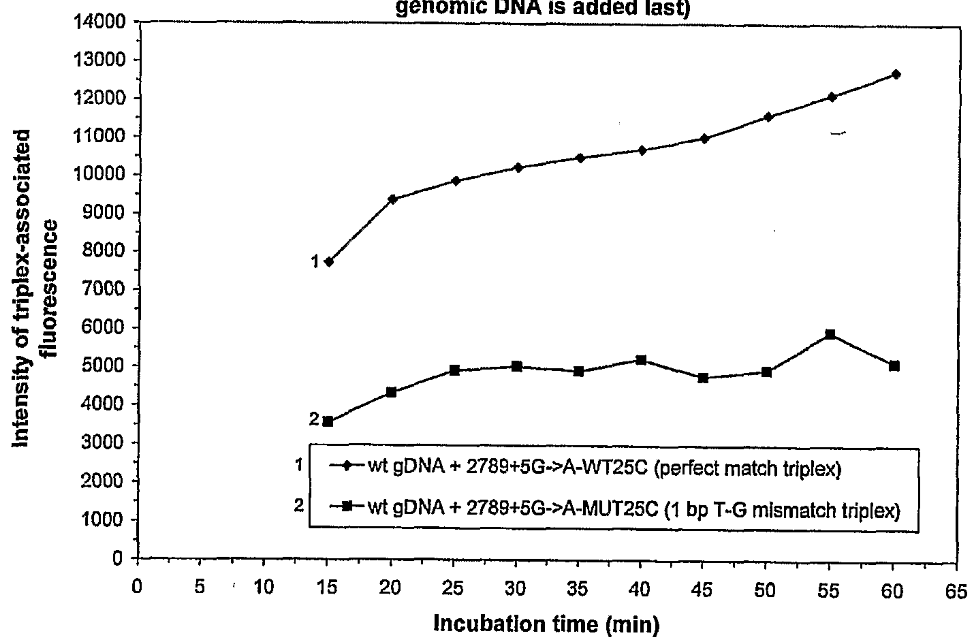
FIG. 2. Triplex-associated fluorescence from human genomic DNA samples assayed in the presence of 500 nM YOYO-1 and 45 mM TMA-Cl (wherein genomic DNA is added last)
