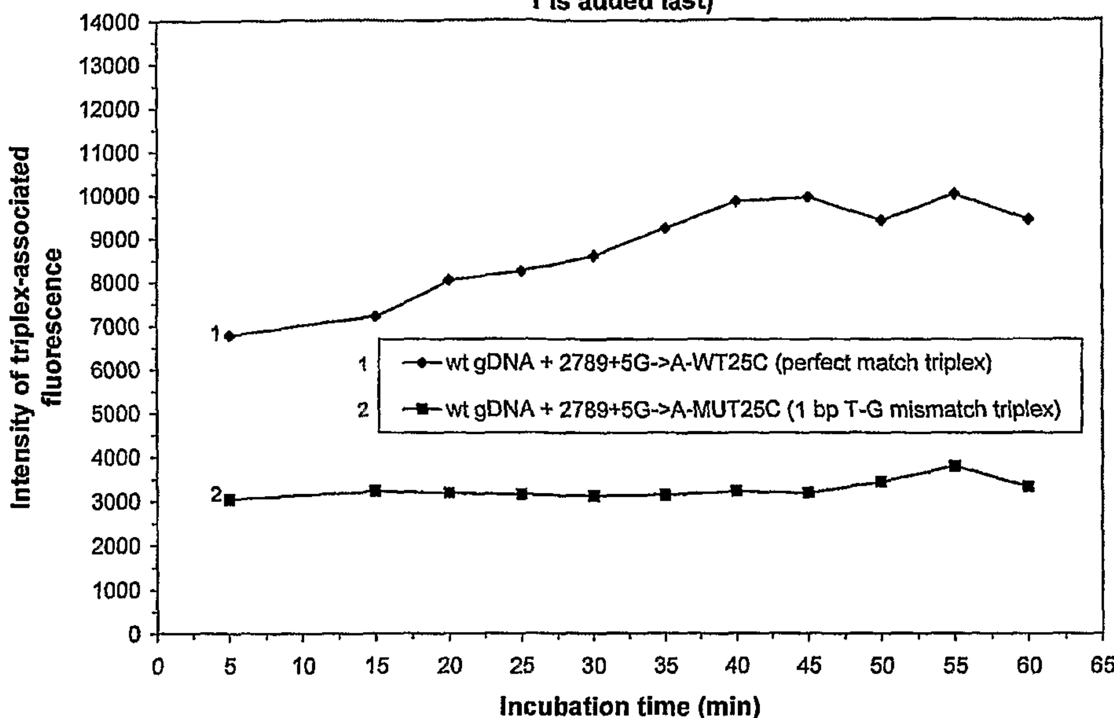
Triplex-associated fluorescence from human genomic DNA samples assayed in the presence of 500 nM YOYO-1 and 45 mM TMA-Cl (wherein YOYO- 1 is added last)
