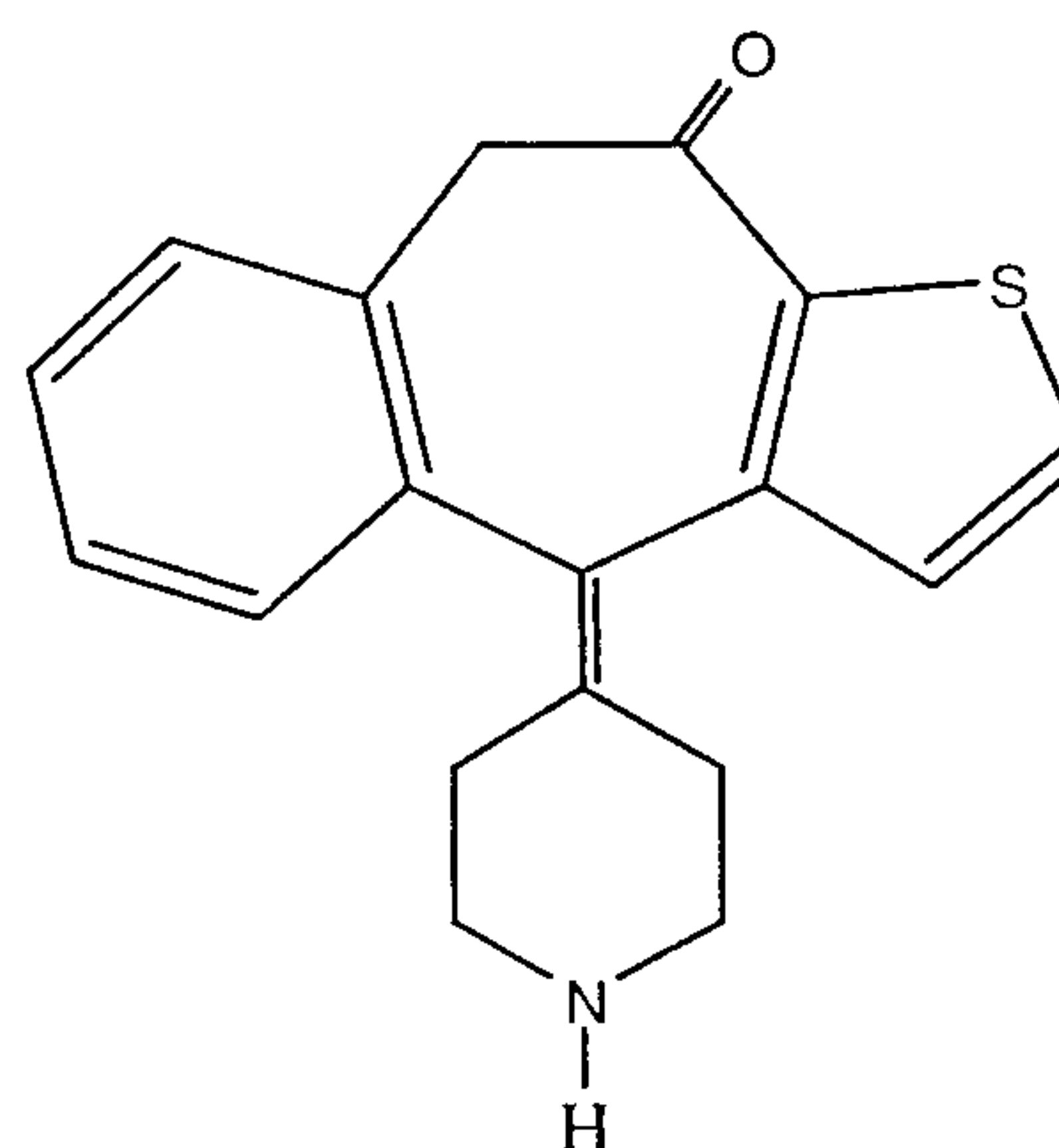
NOR-KETOTIFEN
