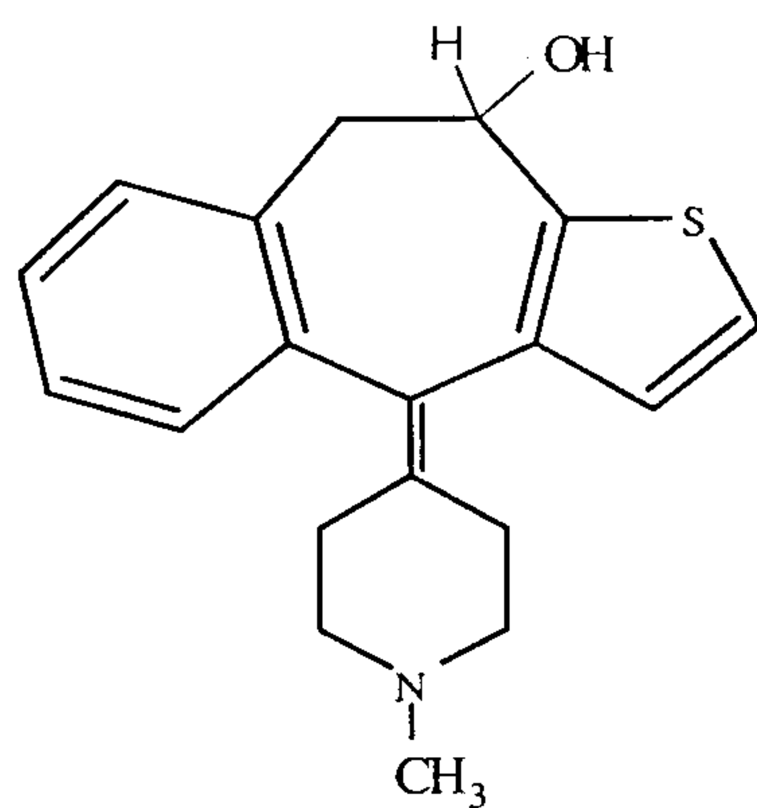
10-HYDROXY-KETOTIFEN
