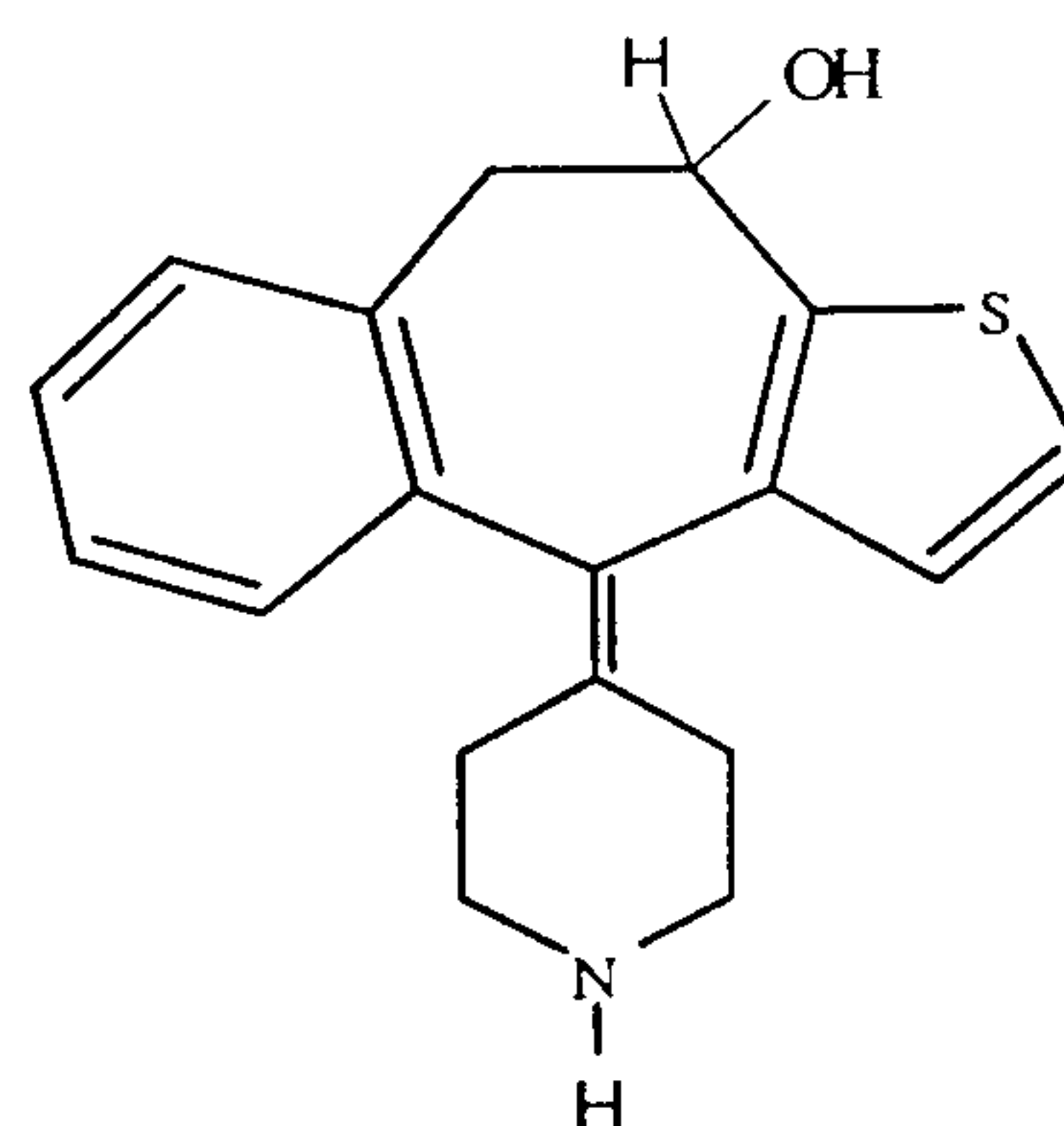
10-HYDROXY-NORKETOTIFEN
