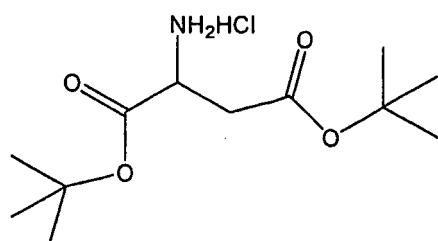
L-aspartic acid di-t-butyl ester hydrochloride
