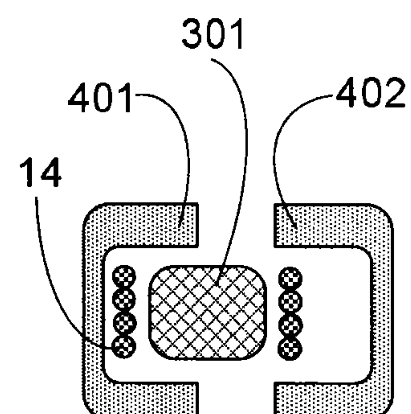
Front View (Cutaway)
