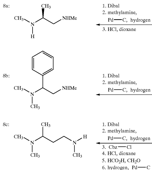
Synthetic Scheme 3
