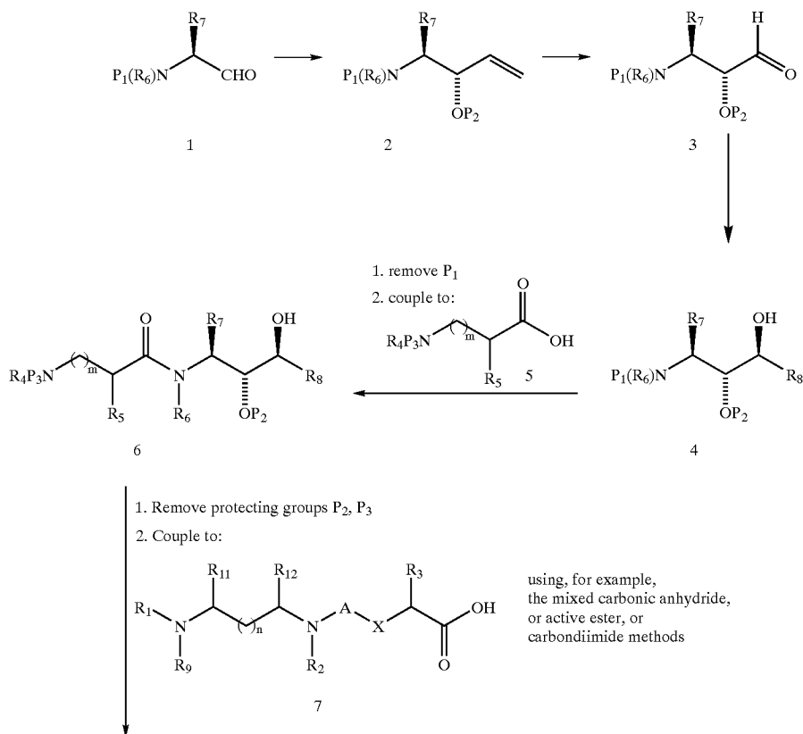
Synthetic Scheme 1
