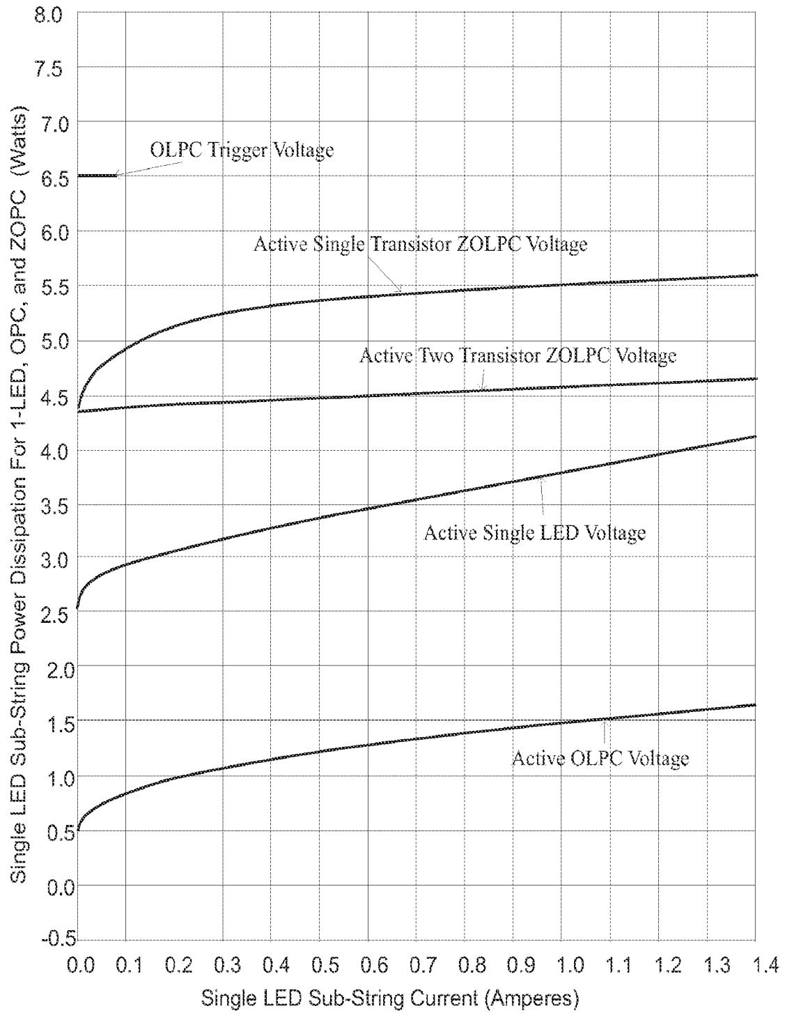
Active Single LED Sub-String For Active I-LED, OLPC, and ZOLPC Voltages versus Current
