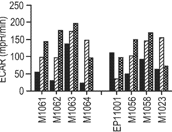
Figure 60E Basal ECAR
