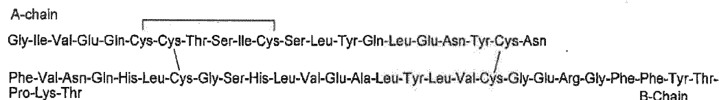
Structure 2 = human Insulin
