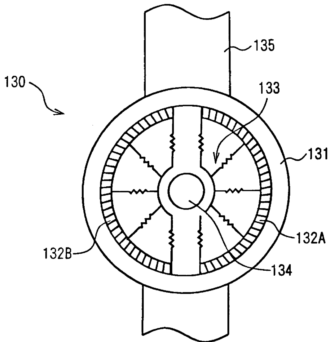
FIG. 2 (RELATED ART)
