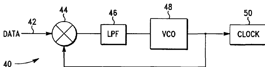
CLOCK RECOVERY FROM DATA STREAM
