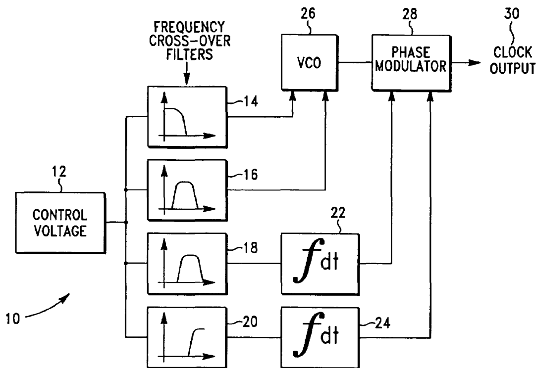
IDEALIZED VOLTAGE CONTROLLED OSCILLATOR
