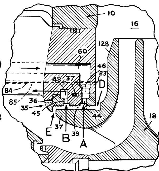
IMPROVED WEARING RING AND SYSTEM FOR REDUCED DILUTION.
