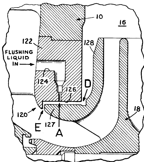
PRIOR ART - WEARING RING WITH CONVENTIONAL FLUSHING.
