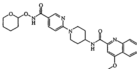
intermediate 3
