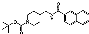
intermediate 4
