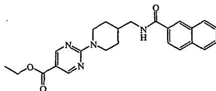
intermediate 6
