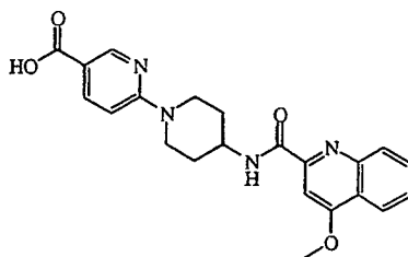
intermediate 2
