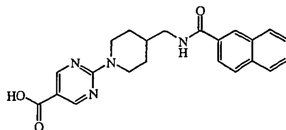
.Na intermediate 7
