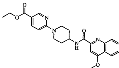
intermediate 1
