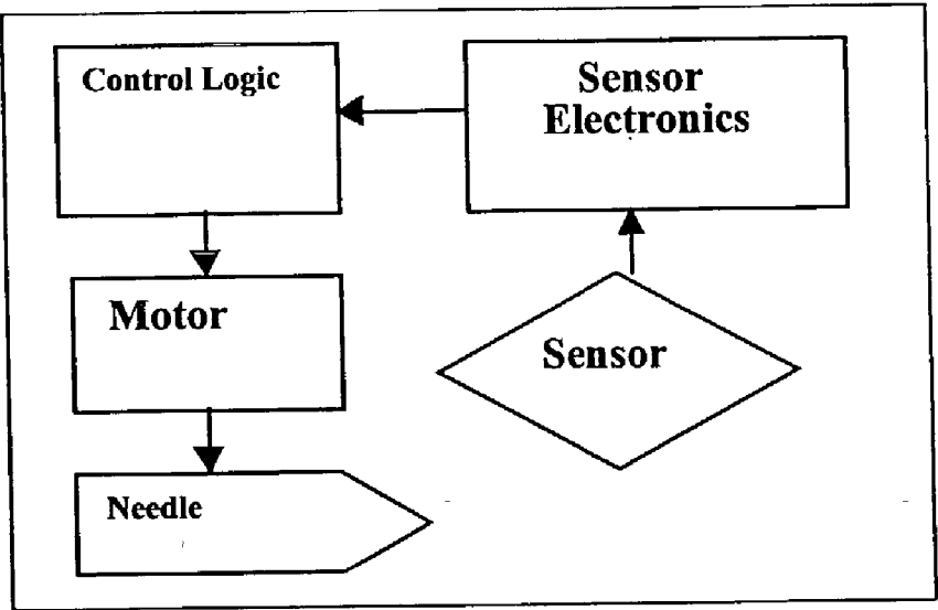
Fig. 21- Feedback loop from blood sensor to Control logic to control depth of microneedle penetration.
