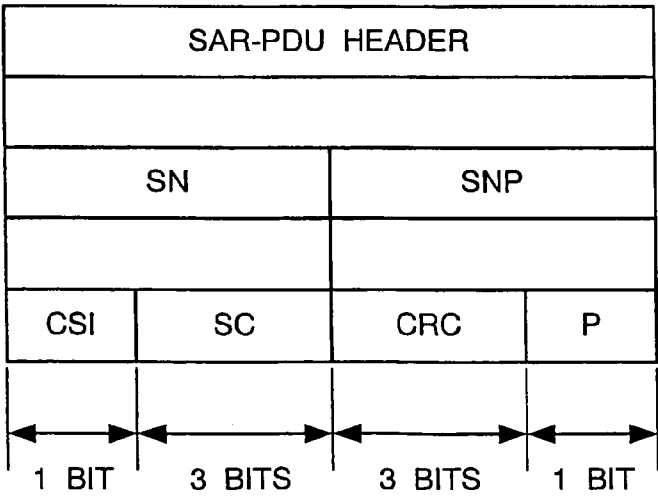
SAR-PDU HEADER FORMAT
