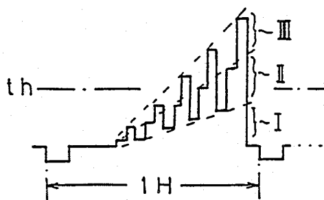
FIG. 1C PRIOR ART
