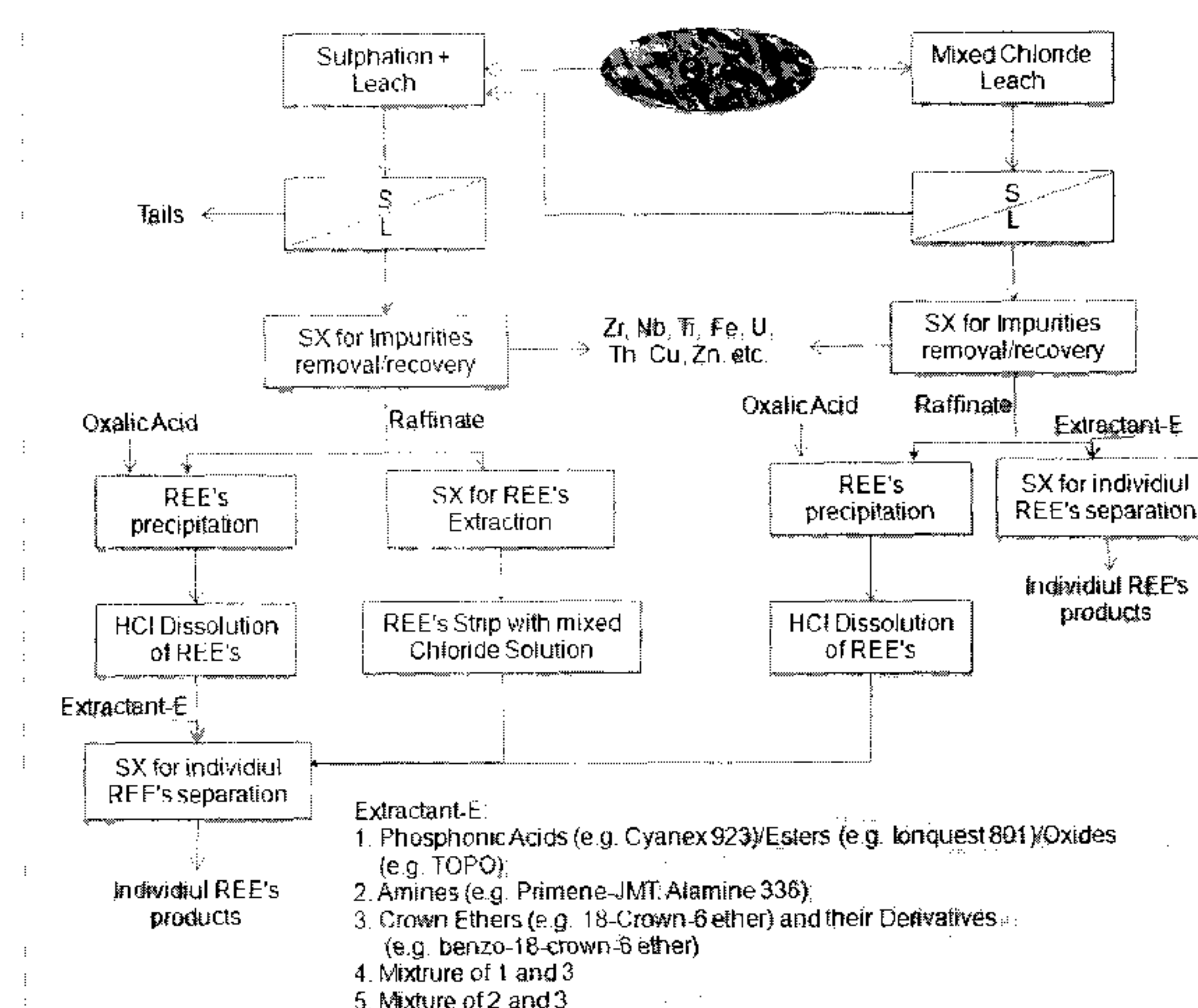
Figure 1 Process flow diagram.
