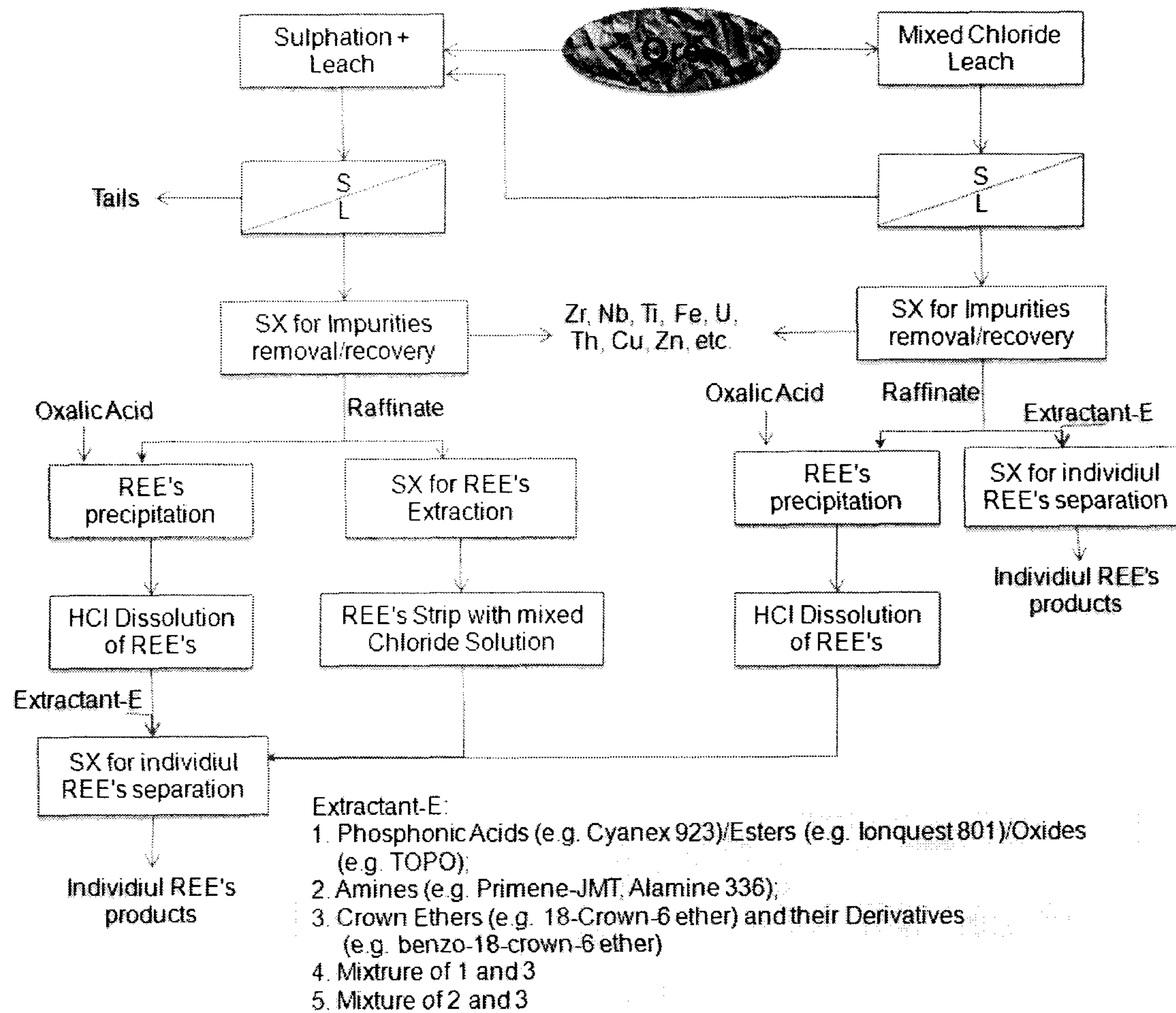
Figure 1 Process flow diagram.
