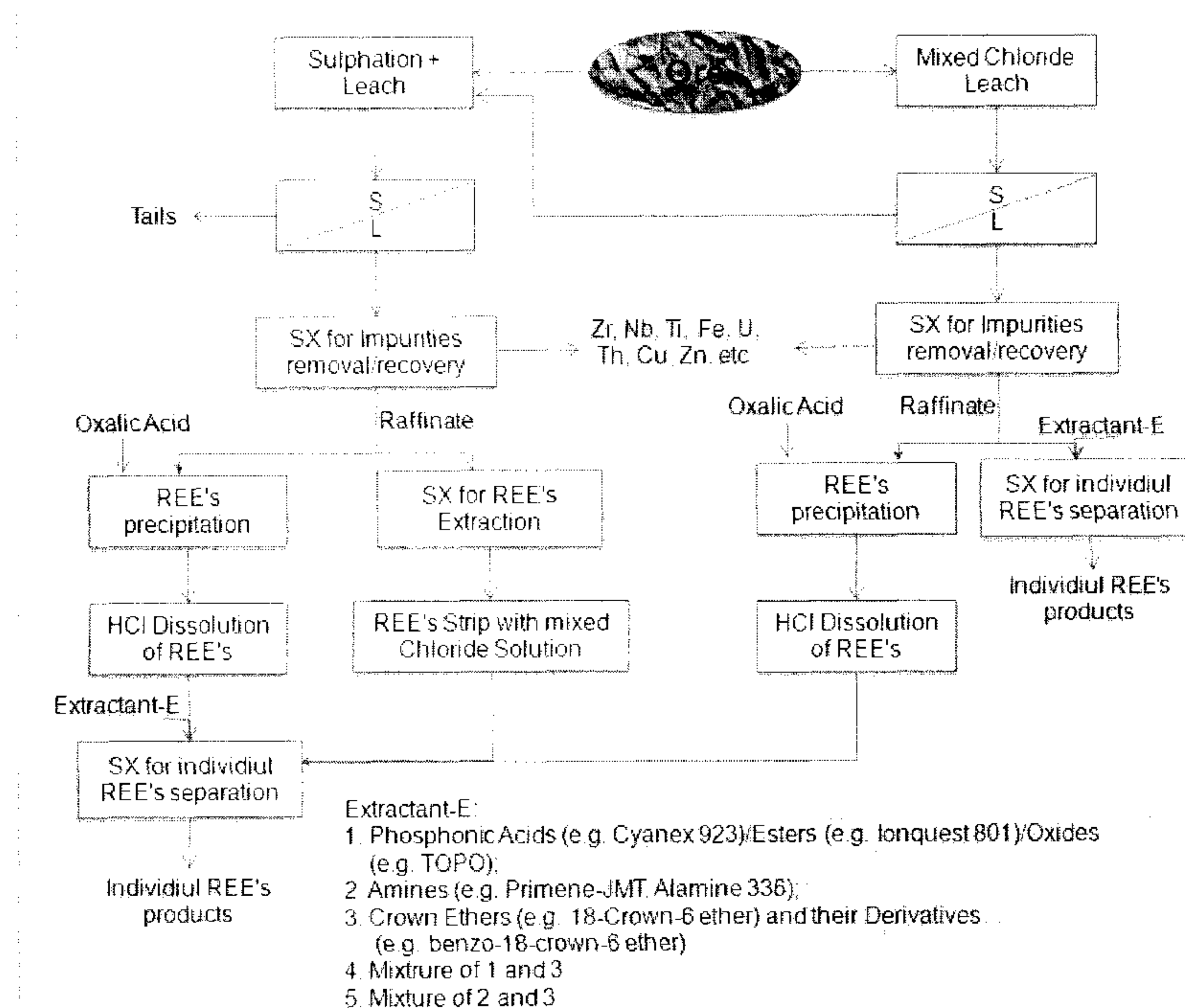
Figure 1 Process flow diagram.
