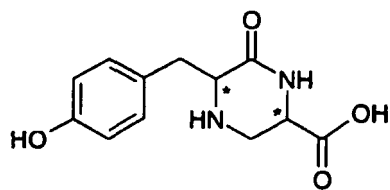
5-(4-Hydroxy-benzyl)-6-oxo-piperazine-2-carboxylic acid
