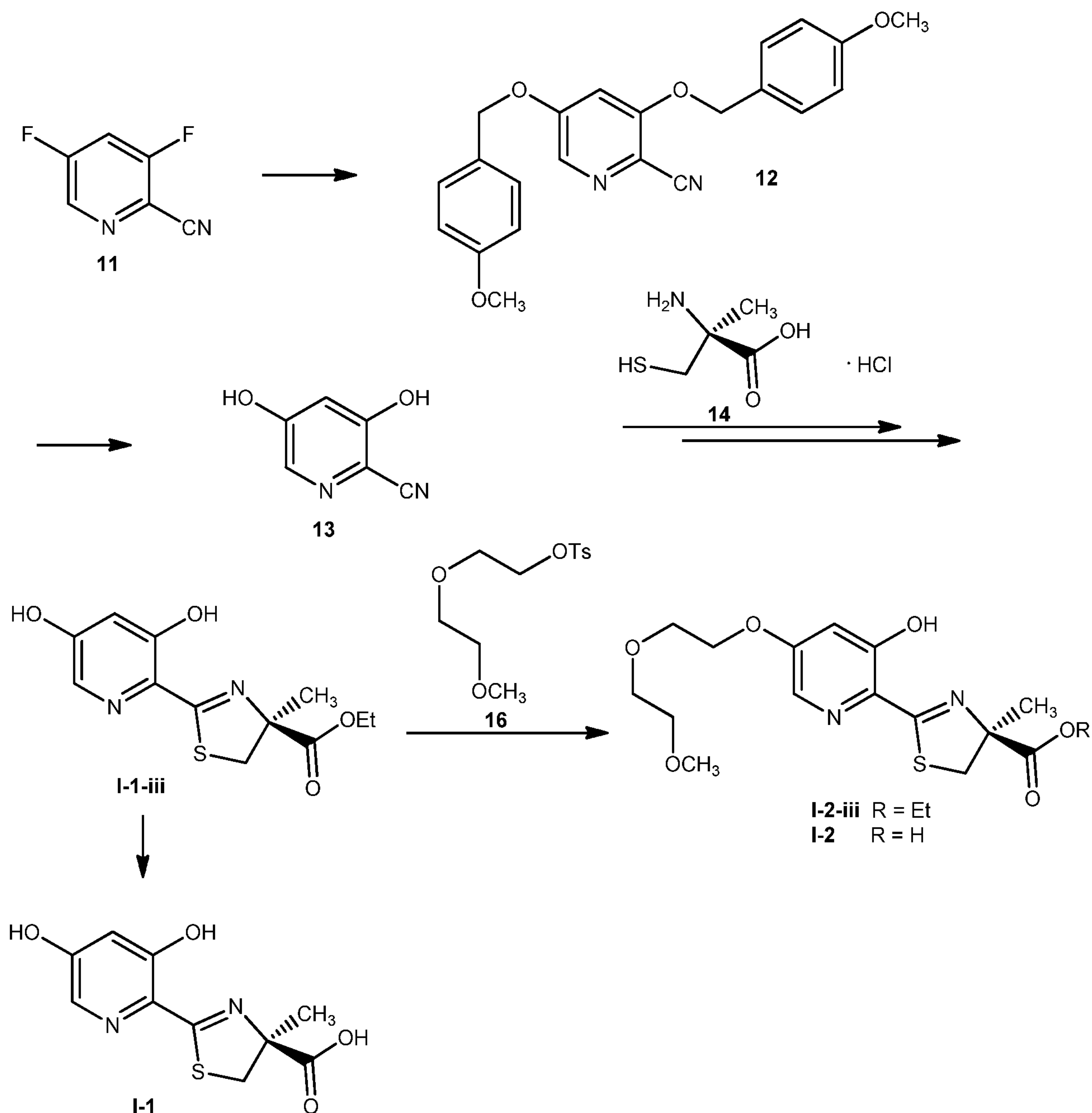
Scheme 1. Exemplary synthesis of I-1 and I-2 .
