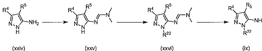
Scheme 7
