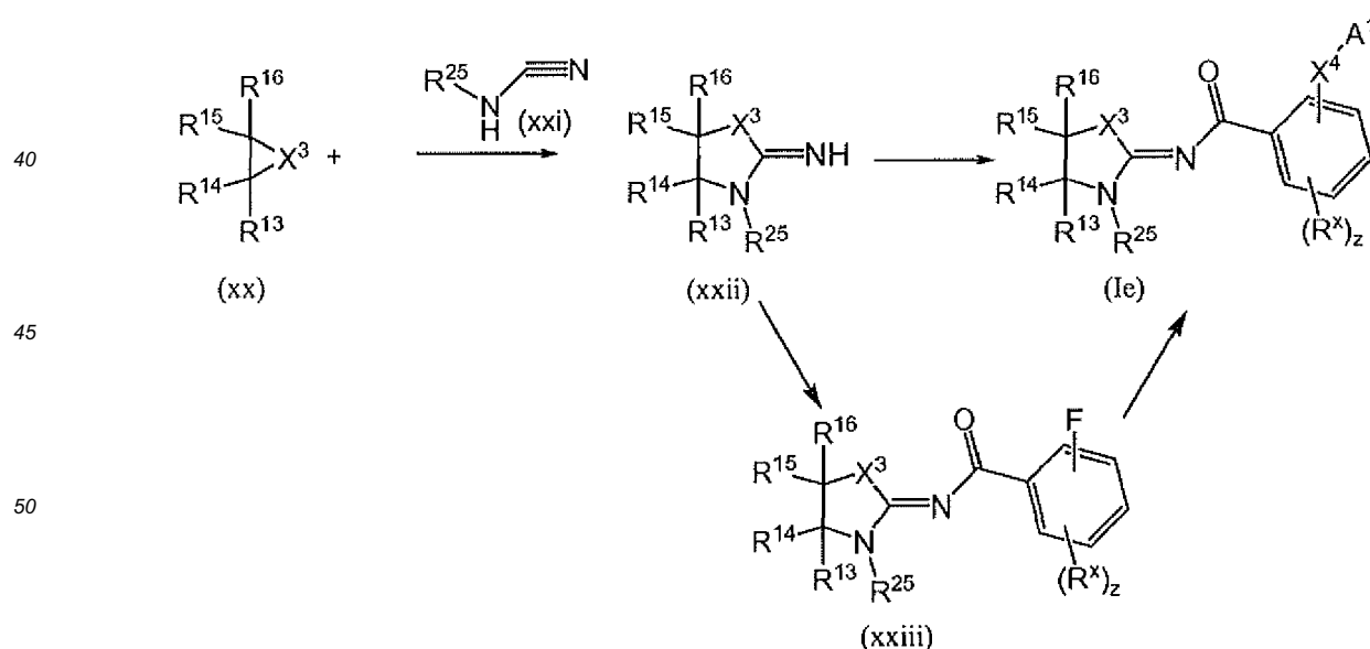
Scheme 6
