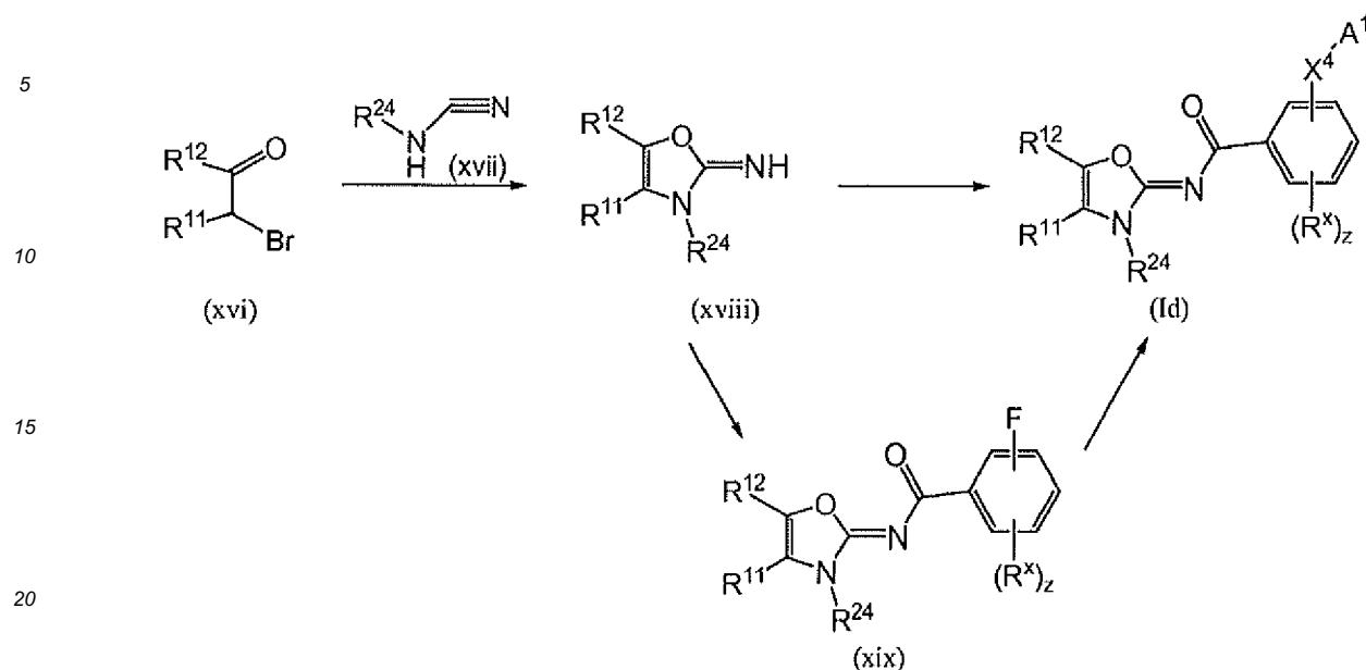
Scheme 5
