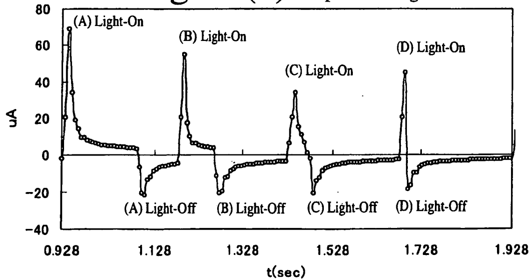
Reference Fig. 18(b) Response to Light in one Turn
