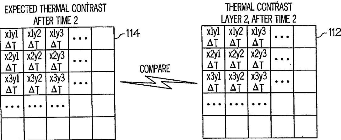
SELF REFERENCING THERMAL CONTRAST PIXEL COMPUTATION LAYER 2, TIME 2
