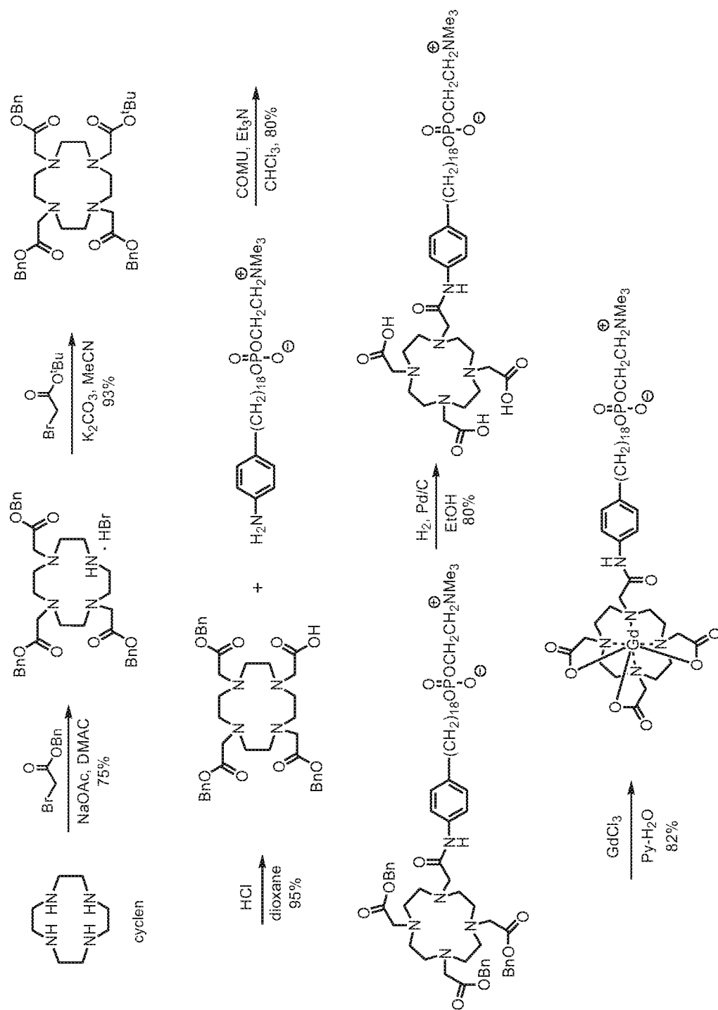
[00118] Scheme for synthesizing Gd-DO3A-404:
