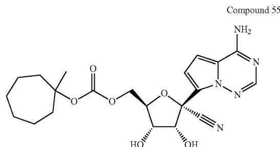
Compound 55
