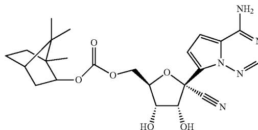
Compound 71
