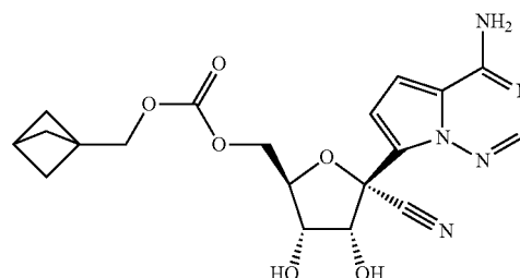
Compound 72
