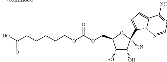
Compound 140
