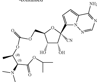
Compound 145
