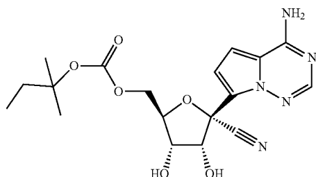
Compound 70
