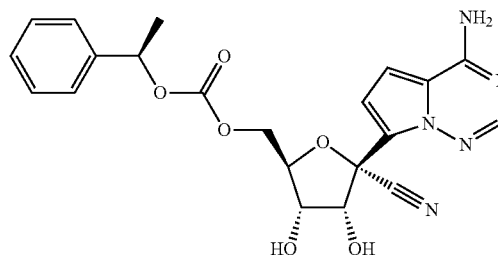
Compound 87
