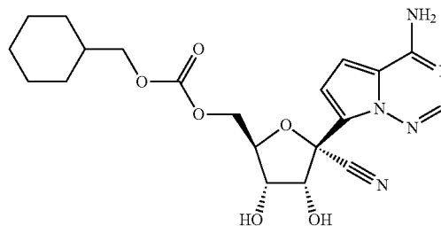
Compound 86
