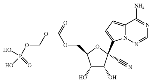
Compound 40
