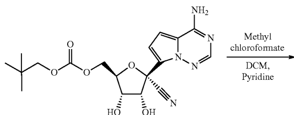
Compound 3
