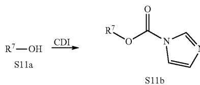
Scheme 11
