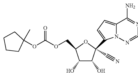
Compound 56
