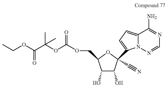
Compound 77
