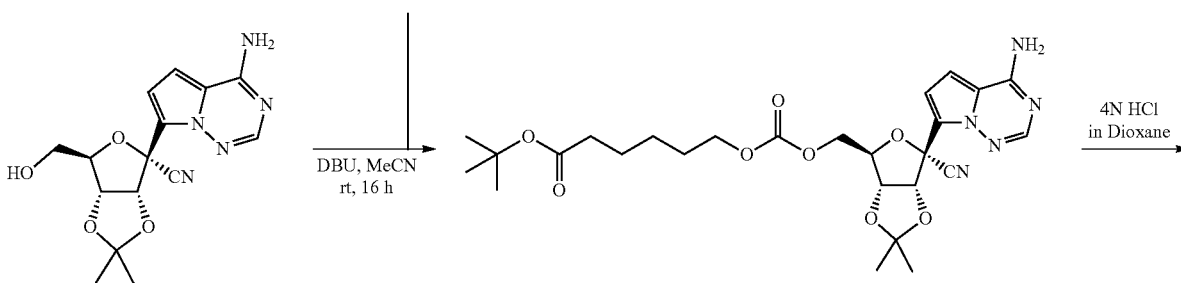
Intermediate I
