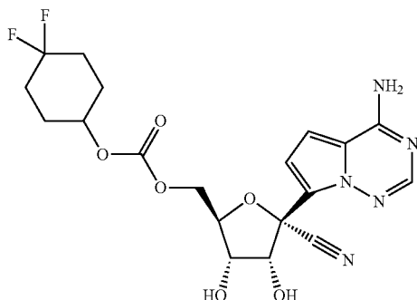
Compound 84
