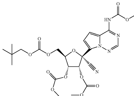
Compound 103
