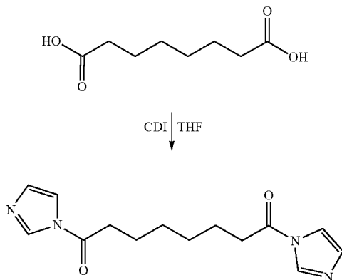
Intermediate 85a
