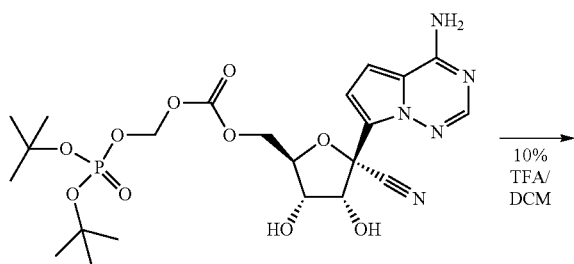
Compound 110
