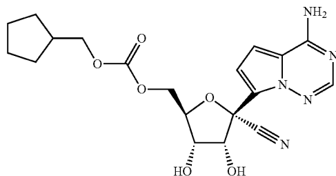
Compound 85
