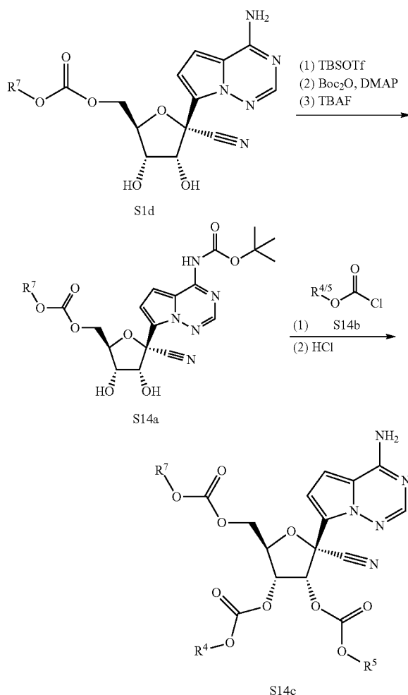
Scheme 14
