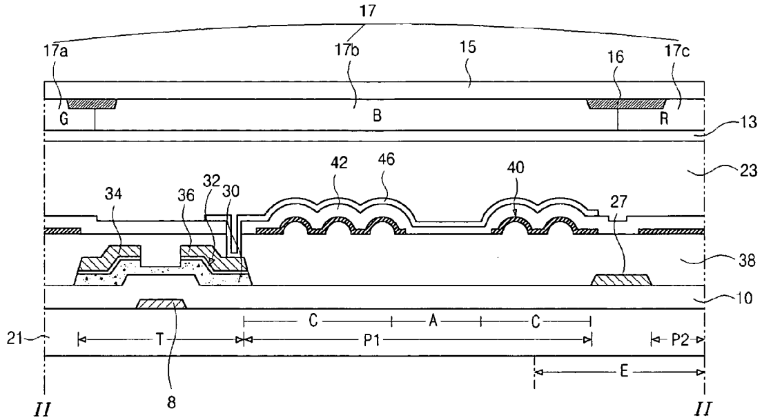
FIG. 2 RELATED ART
