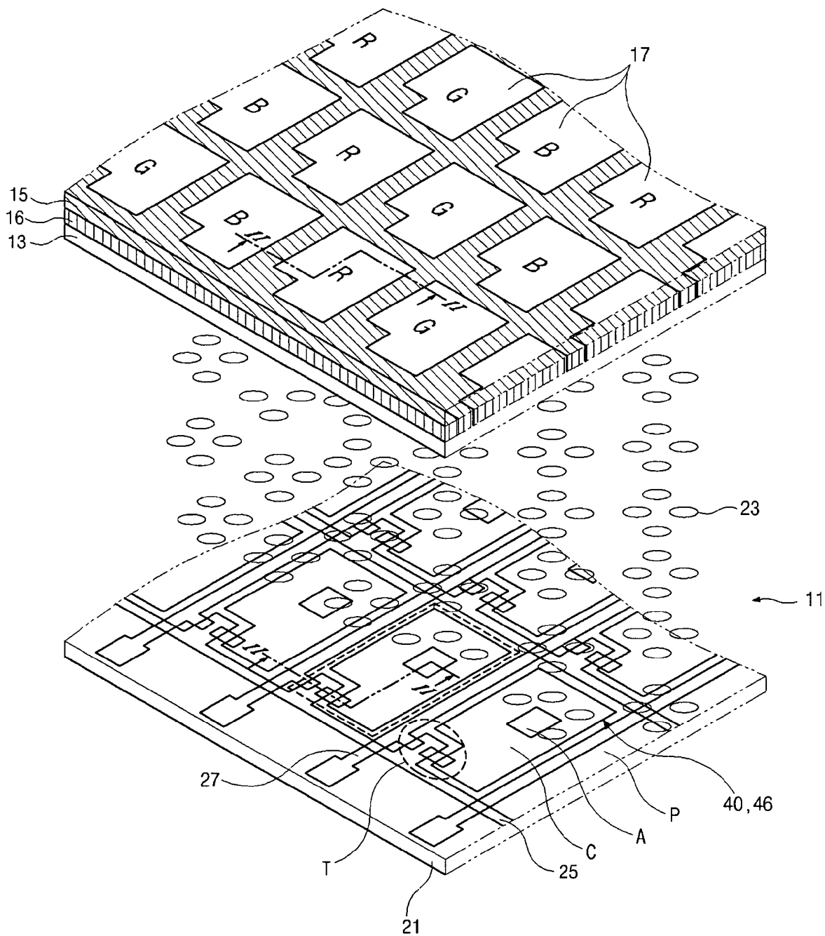
FIG. 1 RELATED ART
