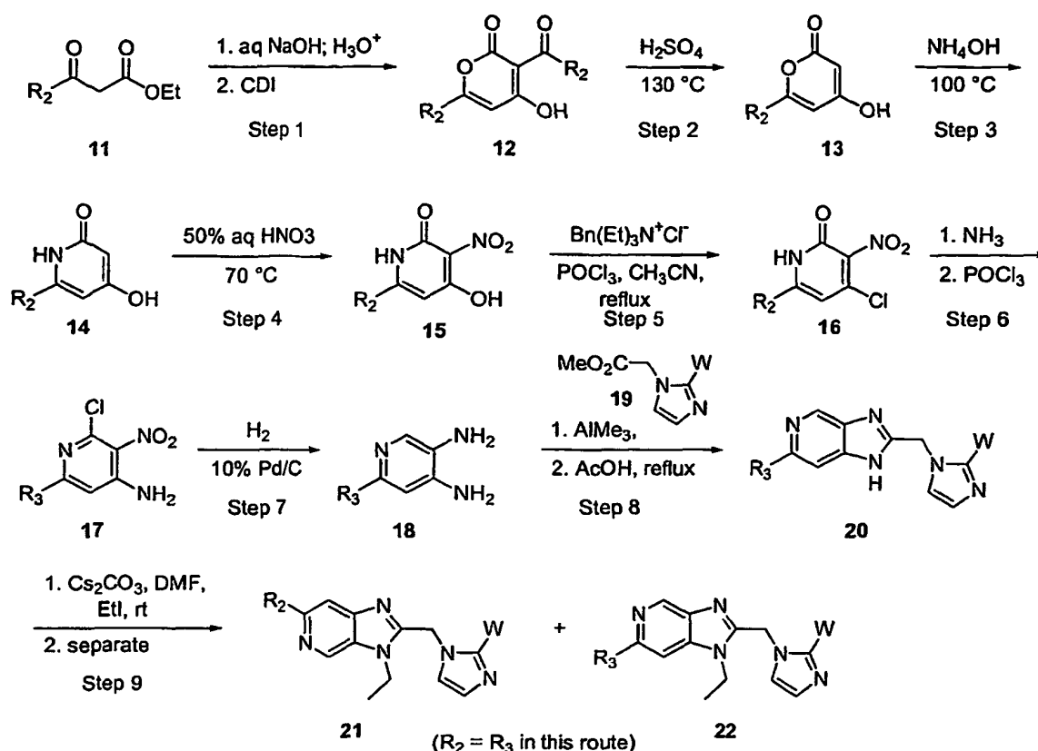
Scheme III
