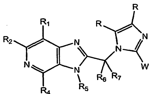
Formula V
