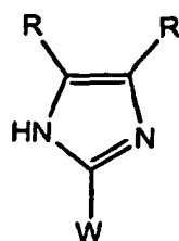
Formula B
