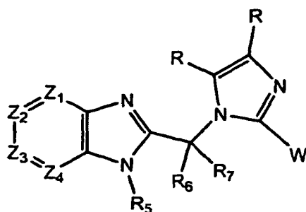
Formula A
