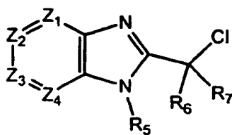
Formula C
