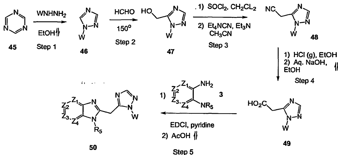
Scheme IX
