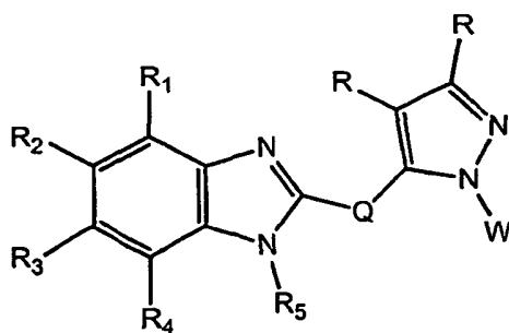
Formula III
