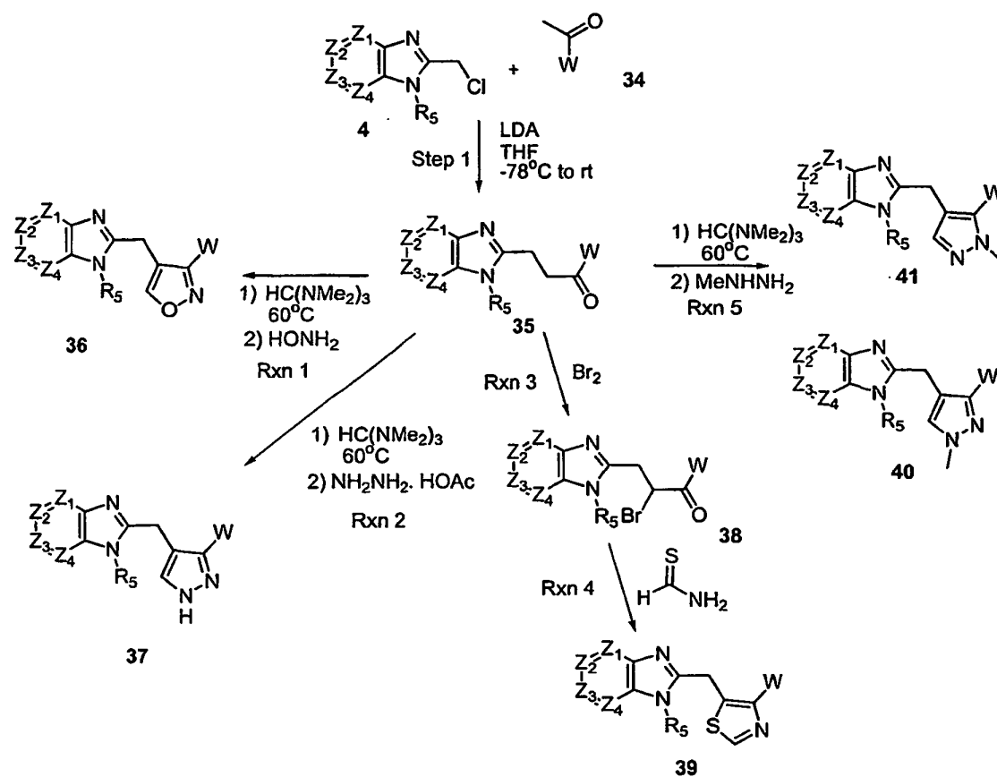
Scheme VII
