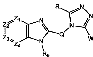
Formula X
