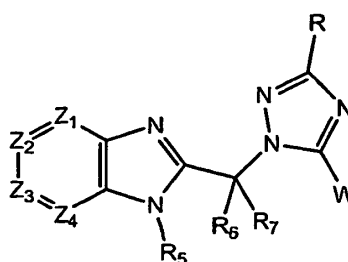
Formula XI
