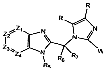
Formel A
