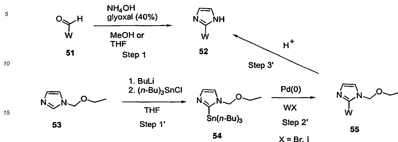
Scheme X
