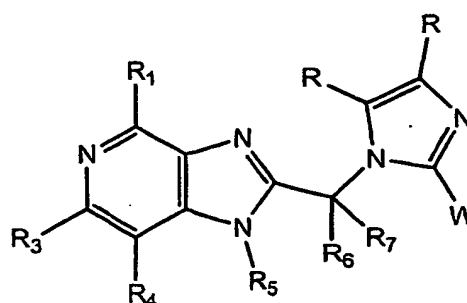
Formula VI
