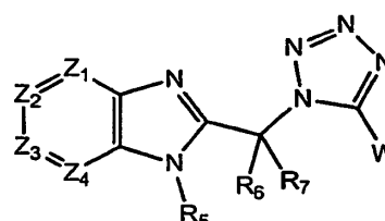
Formula XVIII
