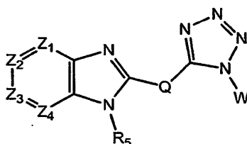
Formula XVII
