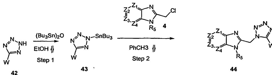
Scheme VIII
