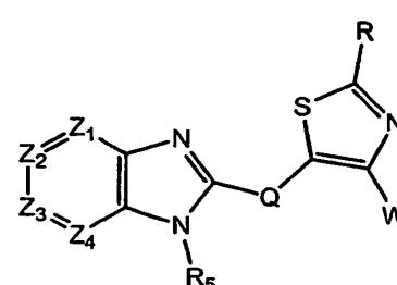
Formula XII
