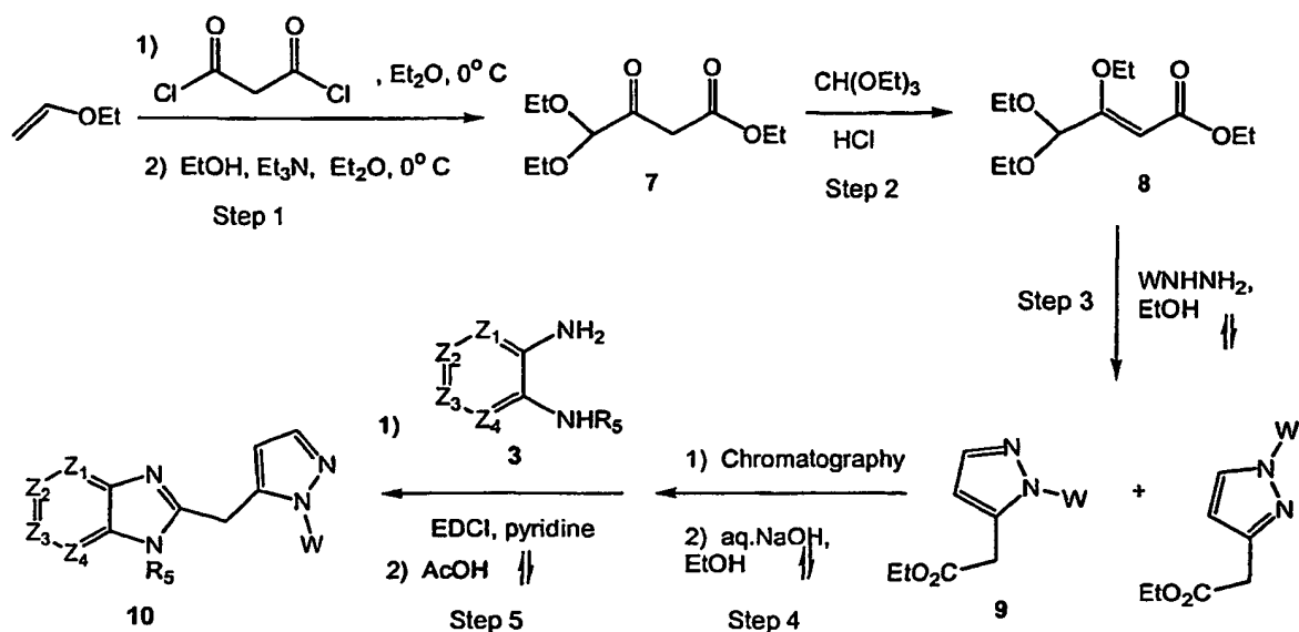
Scheme II
