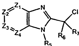
Formel C
