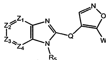
Formula XVI
