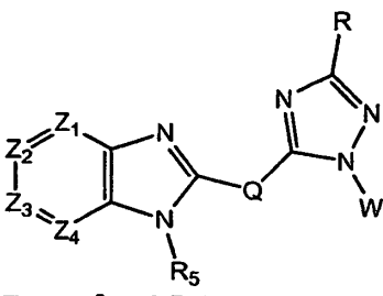
Formula XIV
