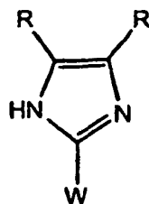
Formel B
