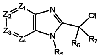
Formula C.
