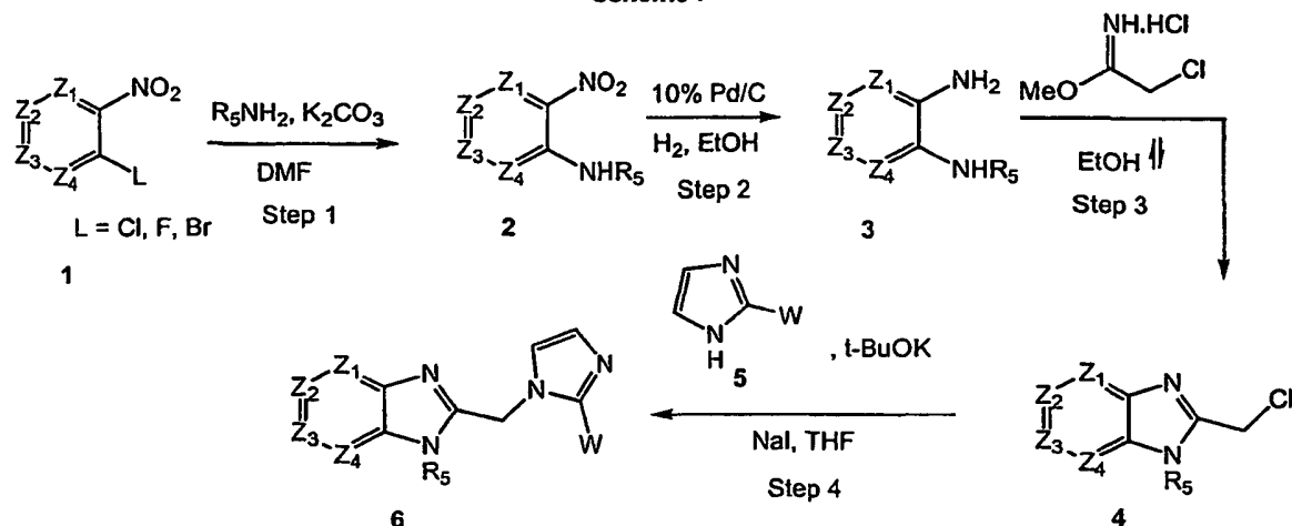
Scheme I
