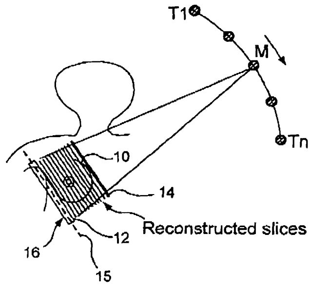
FIG. 3 (previous geometry)
