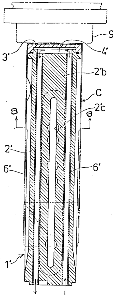
Fig. 7 Prior Art
