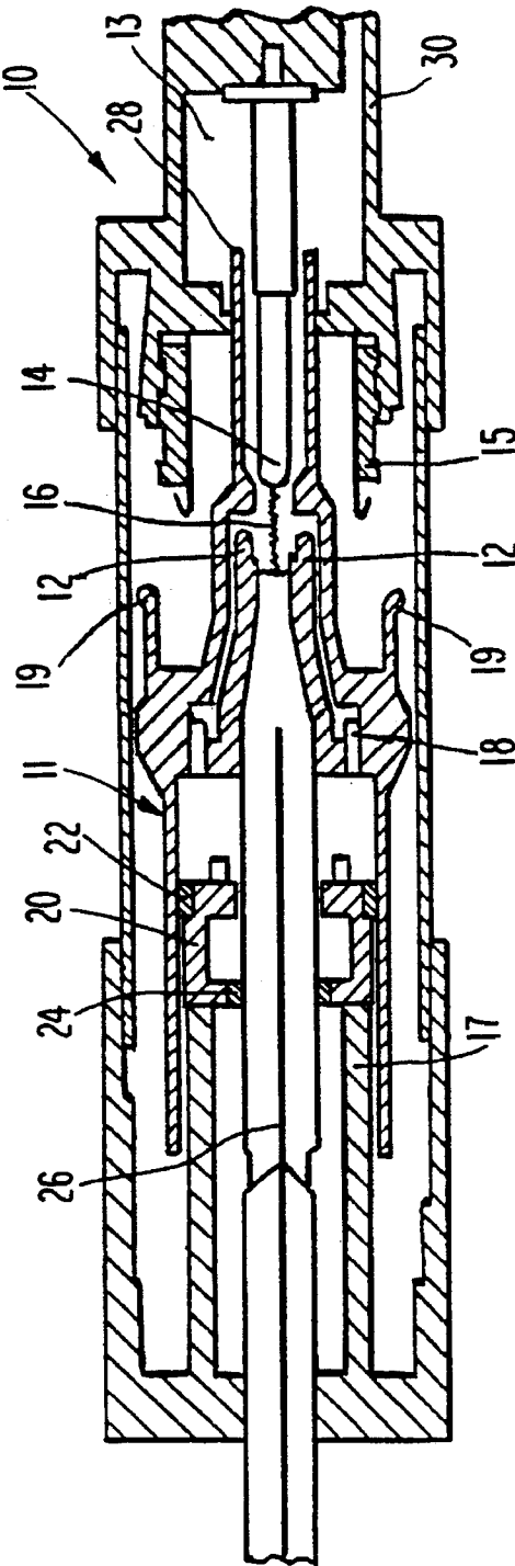
Fig. 2 PRIOR ART
