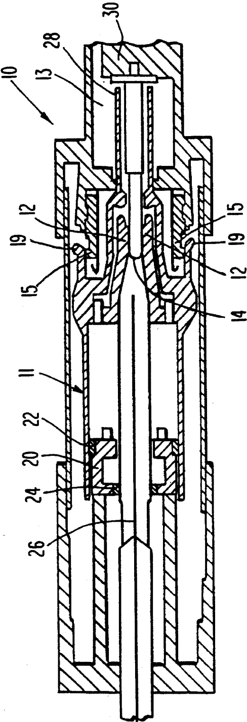
Fig. 1 PRIOR ART
