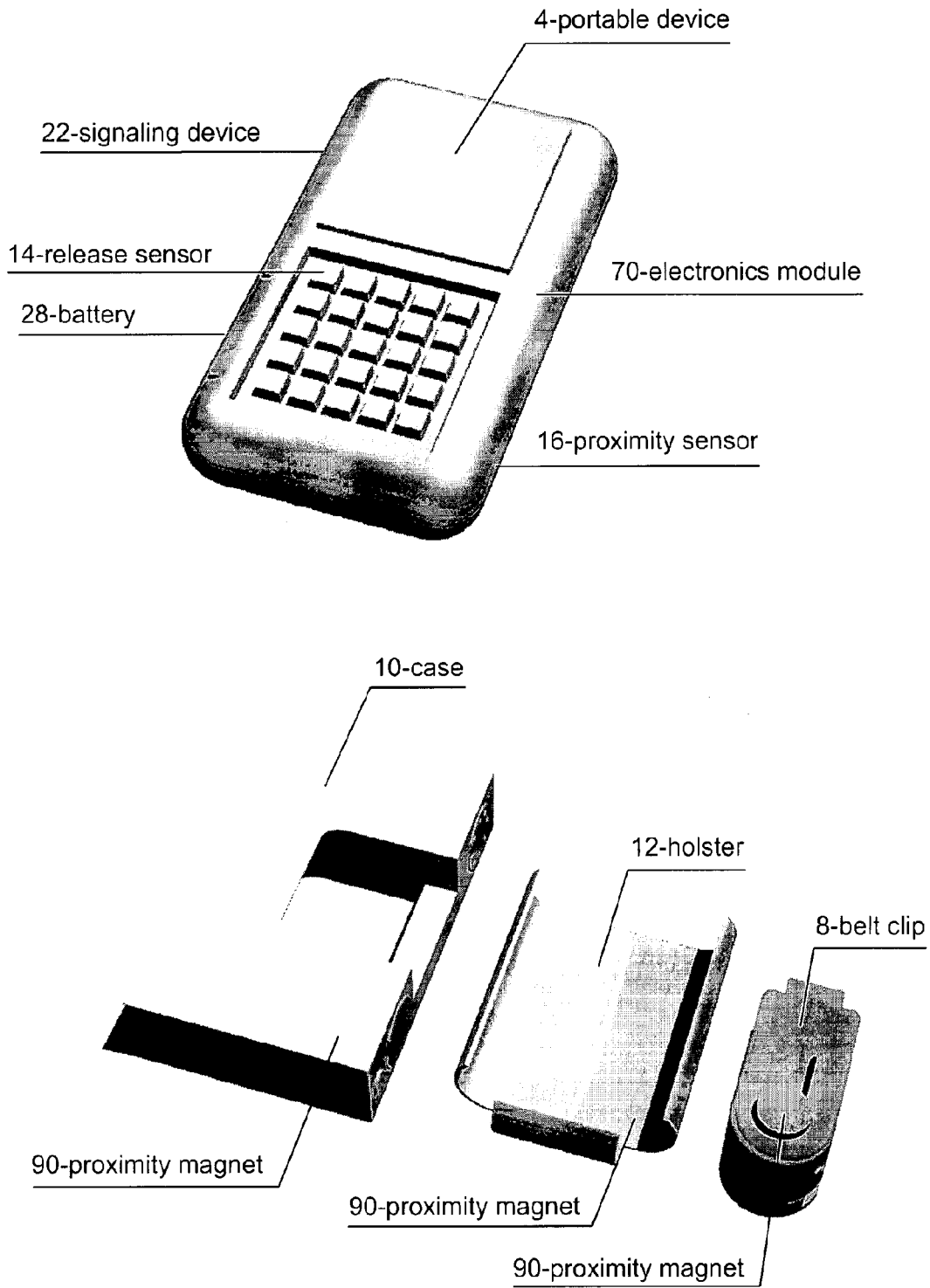
EDF BUILT INTO PORTABLE DEVICE
