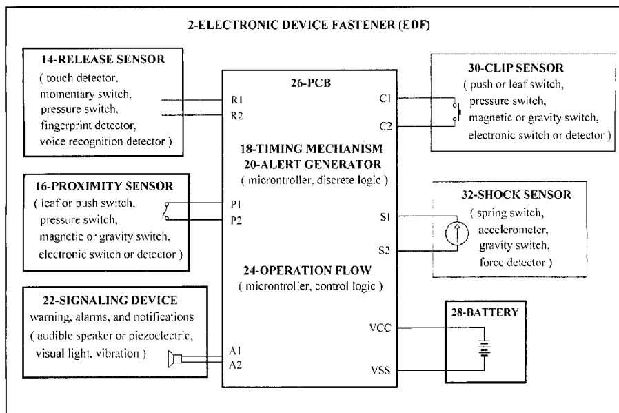
CIRCUIT BLOCK DIAGRAM
