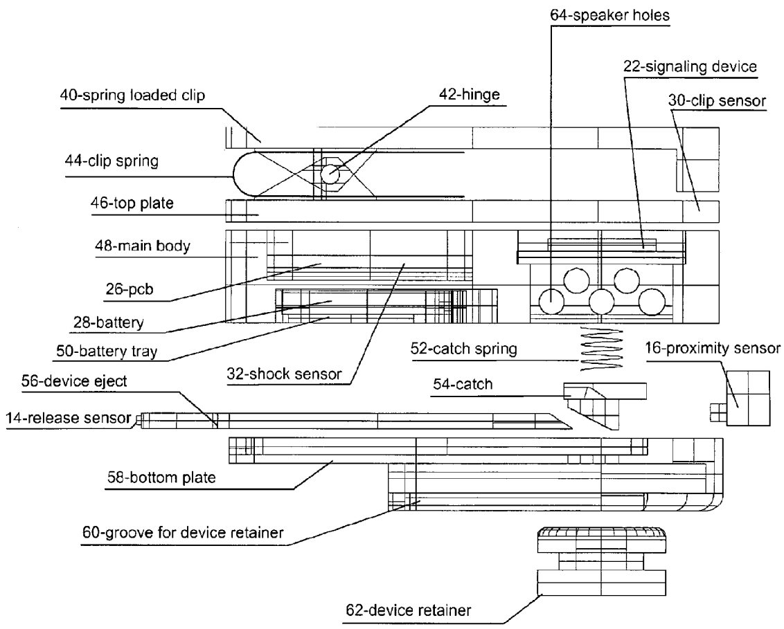
CROSS SECTIONAL VIEW BELT CLIP
