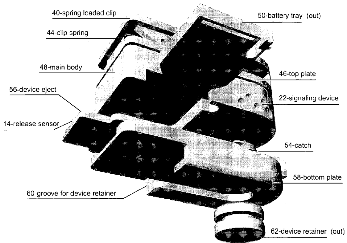
BOTTOM PERSPECTIVE VIEW BELT CLIP
