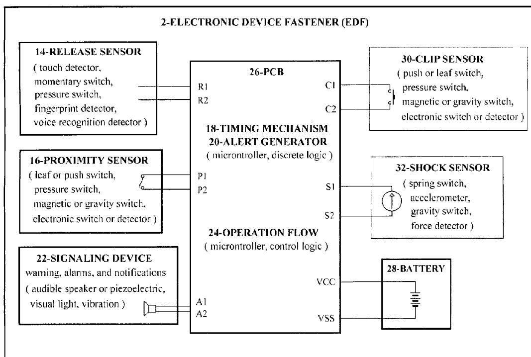
CIRCUIT BLOCK DIAGRAM
