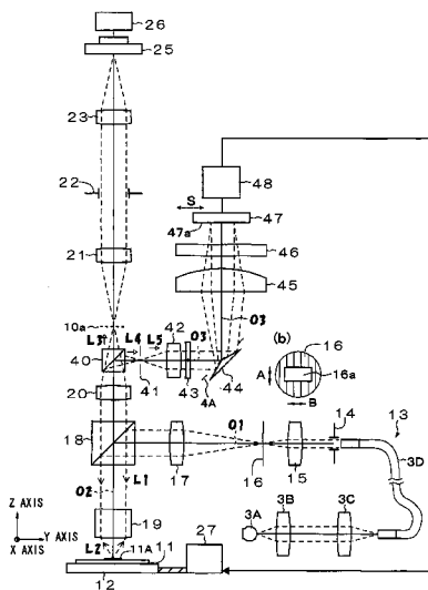
(a) 10 (OVERLAY MEASUREMENT APPARATUS)
