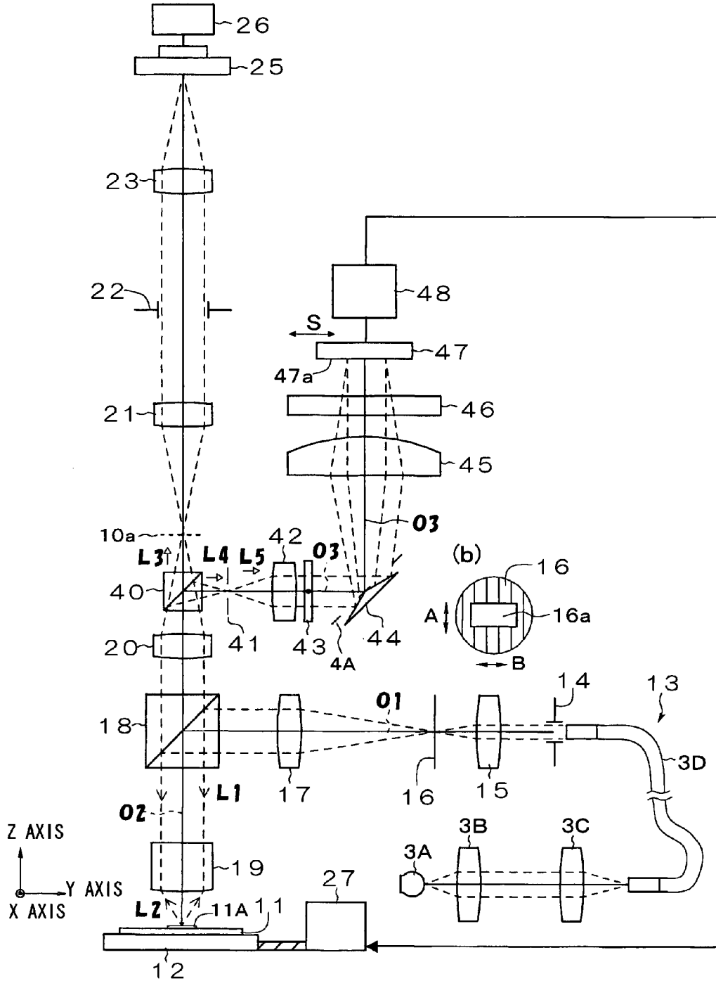
(a) 10 (OVERLAY MEASUREMENT APPARATUS)
