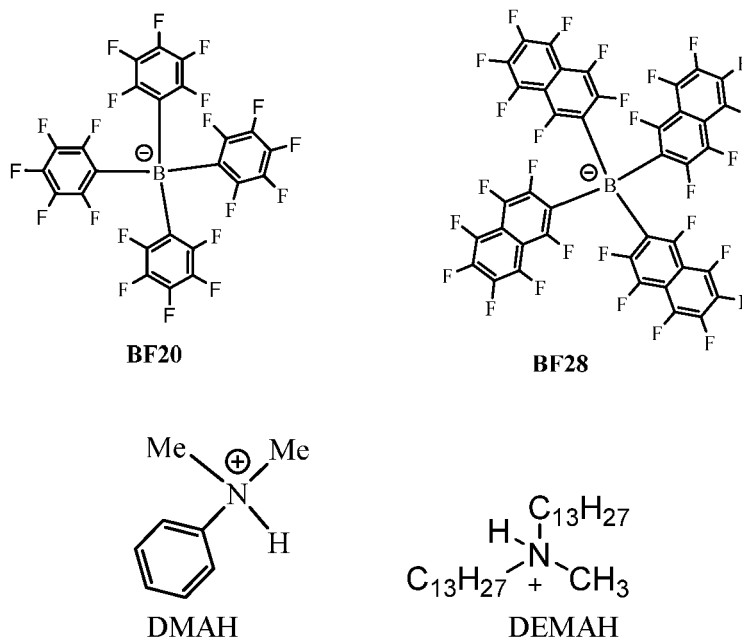
Scheme 1: Borate Anions and Ammonium Cations used as Activator Components.
