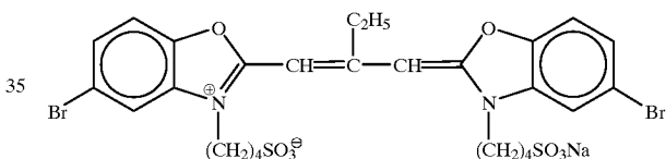
Sensitizing dye 16
