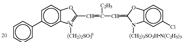
Sensitizing dye 14
