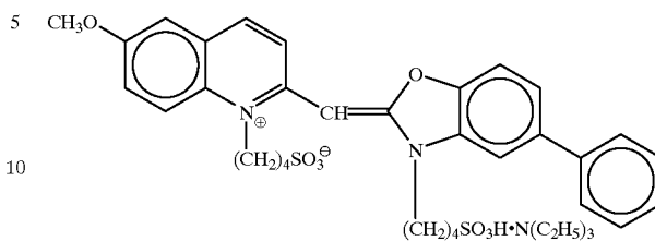
Sensitizing dye 14
