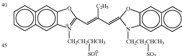
Sensitizing dye 16
