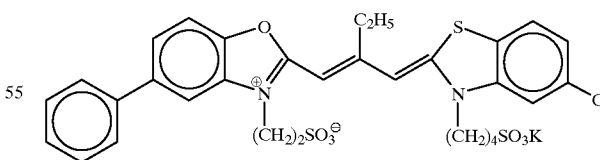
Sensitizing dye 17
