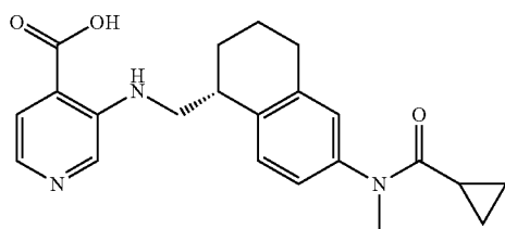
3-({[(1R)-6-(N-methylcyclopropaneamido)-1,2,3,4-tetrahydronaphthalen-1-yl]methyl}amino)pyridine-4-carboxylic acid
