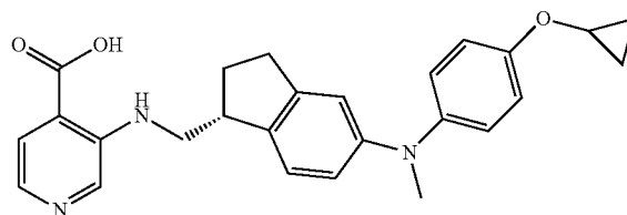
3-({[(1R)-5-{[4-(cyclopropoxy)phenyl](methyl)amino}-2,3-dihydro-1H-inden-1-yl]methyl}amino)pyridine-4-carboxylic acid
