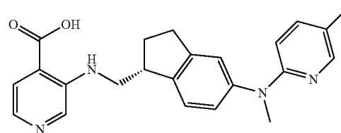
3-({[(1R)-5-[methyl(5-methylpyridin-2-yl)amino]-2,3-dihydro-1H-inden-1-yl]methyl}amino)pyridine-4-carboxylic acid
