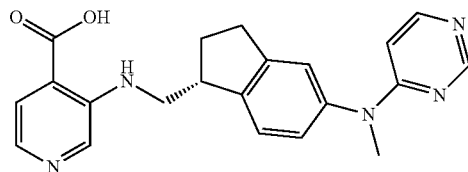
3-({[(1R)-5-[methyl(pyrimidin-4-yl)amino]-2,3-dihydro-1H-inden-1-yl]methyl}amino)pyridine-4-carboxylic acid
