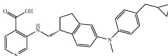
3-({[(1R)-5-{[4-(cyclopropylmethyl)phenyl](methyl)amino}-2,3-dihydro-1H-inden-1-yl]methyl}amino)pyridine-4-carboxylic acid
