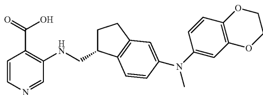
3-({[(1R)-5-[(2,3-dihydro-1,4-benzodioxin-6-yl)(methyl)amino]-2,3-dihydro-1H-inden-1-yl]methyl}amino)pyridine-4-carboxylic acid
