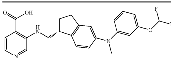
3-({[(1R)-5-{[3-(difluoromethoxy)phenyl](methyl)amino}-2,3-dihydro-1H-inden-1-yl]methyl}amino)pyridine-4-carboxylic acid
