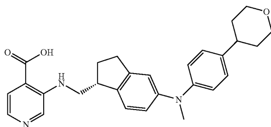
3-({[(1R)-5-[methyl[4-(oxan-4-yl)phenyl]amino]-2,3-dihydro-1H-inden-1-yl]methyl}amino)pyridine-4-carboxylic acid
