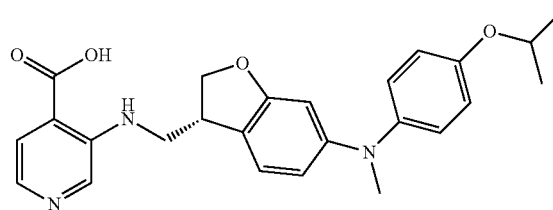
3-({[(3R)-6-{methyl[4-(propan-2-yloxy)phenyl]amino}-2,3-dihydro-1-benzofuran-3-yl]methyl}amino)pyridine-4-carboxylic acid
