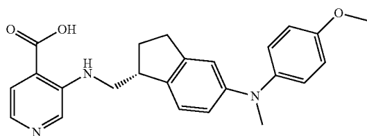
3-({[(1R)-5-{(4-methoxyphenyl)(methyl)amino}-2,3-dihydro-1H-inden-1-yl]methyl}amino)pyridine-4-carboxylic acid
