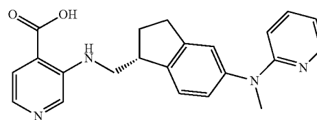
3-({[(1R)-5-{methyl(pyridin-2-yl)amino}-2,3-dihydro-1H-inden-1-yl]methyl}amino)pyridine-4-carboxylic acid
