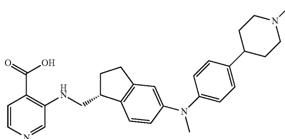
3-({[(1R)-5-[methyl[4-(1-methylpiperidin-4-yl)phenyl]amino]-2,3-dihydro-1H-inden-1-yl]methyl}amino)pyridine-4-carboxylic acid
