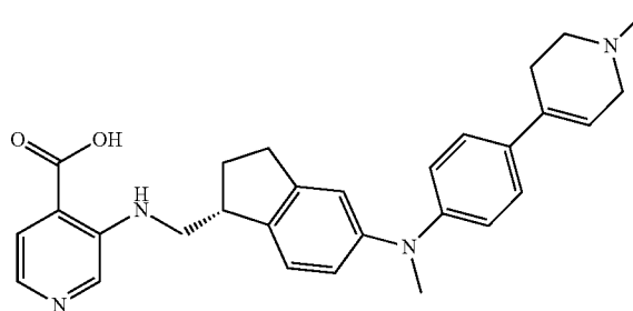
3-({[(1R)-5-[methyl[4-(1-methyl-1,2,3,6-tetrahydropyridin-4-yl)phenyl]amino]-2,3-dihydro-1H-inden-1-yl]methyl}amino)pyridine-4-carboxylic acid
