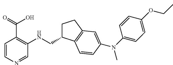
3-({[(1R)-5-{(4-methoxyphenyl)(methyl)amino}-2,3-dihydro-1H-inden-1-yl]methyl}amino)pyridine-4-carboxylic acid
