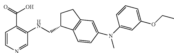
3-({[(1R)-5-{(3-ethoxyphenyl)(methyl)amino}-2,3-dihydro-1H-inden-1-yl]methyl}amino)pyridine-4-carboxylic acid
