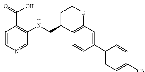
3-({[(4S)-7-(4-cyanophenyl)-3,4-dihydro-2H-1-benzopyran-4-yl]methyl}amino)pyridine-4-carboxylic acid
