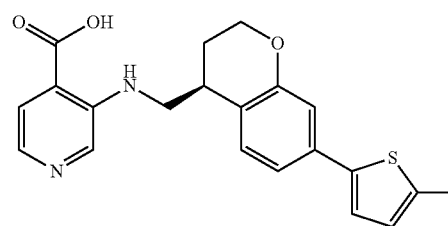
3-({[(4S)-7-(5-methylthiophen-2-yl)-3,4-dihydro-2H-1-benzopyran-4-yl]methyl}amino)pyridine-4-carboxylic acid
