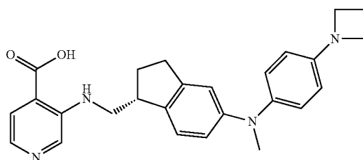
3-({[(1R)-5-{[4-(azetidin-1-yl)phenyl](methyl)amino}-2,3-dihydro-1H-inden-1-yl]methyl}amino)pyridine-4-carboxylic acid
