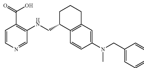
3-({[(1R)-6-[benzyl(methyl)amino]-1,2,3,4-tetrahydronaphthalen-1-yl]methyl}amino)pyridine-4-carboxylic acid
