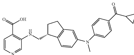
3-({[(1R)-5-{[4-(cyclopropanecarbonyl)phenyl](methyl)amino}-2,3-dihydro-1H-inden-1-yl]methyl}amino)pyridine-4-carboxylic acid
