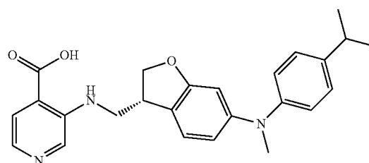
3-({[(3R)-6-{methyl[4-(propan-2-yl)phenyl]amino}-2,3-dihydro-1-benzofuran-3-yl]methyl}amino)pyridine-4-carboxylic acid
