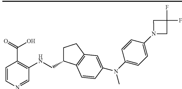
3-({[(1R)-5-{[4-(3,3-difluoroazetidin-1-yl)phenyl](methyl)amino}-2,3-dihydro-1H-inden-1-yl]methyl}amino)pyridine-4-carboxylic acid
