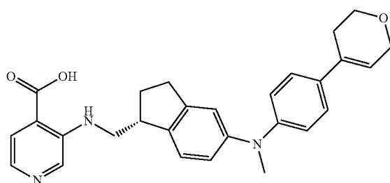
3-({[(1R)-5-[4-(3,6-dihydro-2H-pyran-4-yl)phenyl](methyl)amino]-2,3-dihydro-1H-inden-1-yl]methyl}amino)pyridine-4-carboxylic acid
