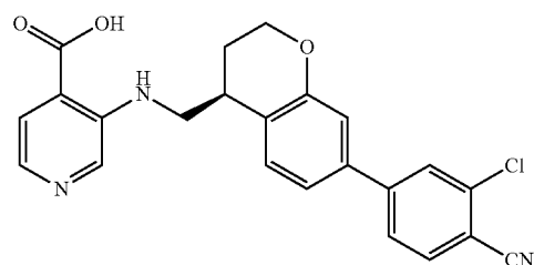
3-({[(4S)-7-(2-chloro-4-cyanophenyl)-3,4-dihydro-2H-1-benzopyran-4-yl)methyl}amino)pyridine-4-carboxylic acid
