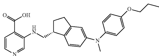
3-({[(1R)-5-{methyl[4-(propoxy)phenyl]amino}-2,3-dihydro-1H-inden-1-yl]methyl}amino)pyridine-4-carboxylic acid
