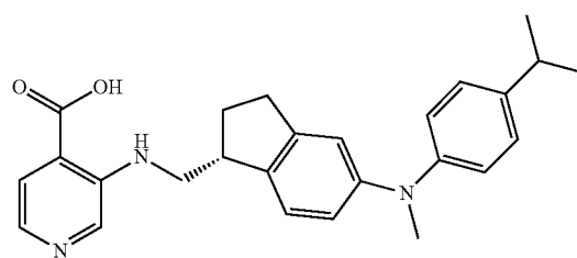
3-({[(1R)-5-{methyl[4-(propan-2-yl)phenyl]amino}-2,3-dihydro-1H-inden-1-yl]methyl}amino)pyridine-4-carboxylic acid
