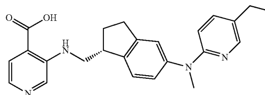
3-({[(1R)-5-[(5-ethylpyridin-2-yl)(methyl)amino]-2,3-dihydro-1H-inden-1-yl]methyl}amino)pyridine-4-carboxylic acid
