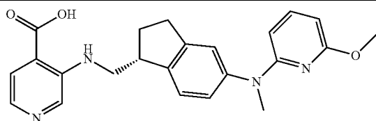
3-({[(1R)-5-[(6-methoxypyridin-2-yl)(methyl)amino]-2,3-dihydro-1H-inden-1-yl]methyl}amino)pyridine-4-carboxylic acid
