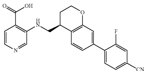
3-({[(4S)-7-(4-cyano-2-fluorophenyl)-3,4-dihydro-2H-1-benzopyran-4-yl)methyl}amino)pyridine-4-carboxylic acid
