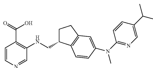
3-({[(1R)-5-{methyl[5-(propan-2-yl)pyridin-2-yl]amino}-2,3-dihydro-1H-inden-1-yl]methyl}amino)pyridine-4-carboxylic acid
