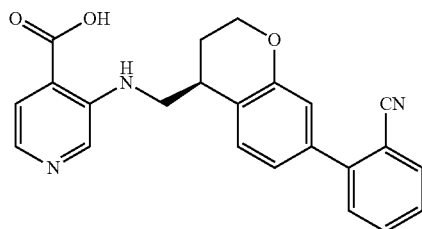
3-({[(4S)-7-(2-cyanophenyl)-3,4-dihydro-2H-1-benzopyran-4-yl)methyl}amino)pyridine-4-carboxylic acid
