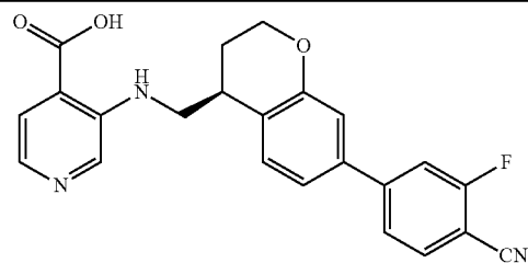
3-({[(4S)-7-(4-cyano-3-fluorophenyl)-3,4-dihydro-2H-1-benzopyran-4-yl)methyl}amino)pyridine-4-carboxylic acid
