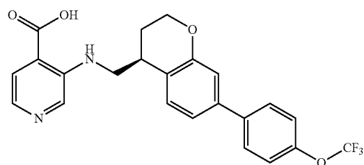
3-({[(4S)-7-[4-(trifluoromethoxy)phenyl]-3,4-dihydro-2H-1-benzopyran-4-yl)methyl}amino)pyridine-4-carboxylic acid
