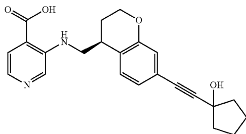
3-({[(4S)-742-(1-hydroxycyclopentyl)ethynyl]-3,4-dihydro-2H-1-benzopyran-4-yl)methyl}amino)pyridine-4-carboxylic acid
