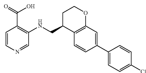
3-({[(4S)-7-(4-chlorophenyl)-3,4-dihydro-2H-1-benzopyran-4-yl)methyl}amino)pyridine-4-carboxylic acid
