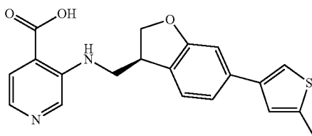
3-({[(3S)-6-(5-methylthiophen-3-yl)-2,3-dihydro-1-benzofuran-3-yl]methyl}amino)pyridine-4-carboxylic acid
