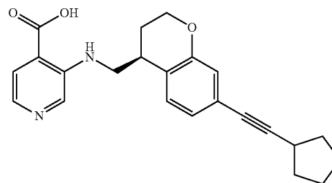
3-({[(4S)-7-(2-cyclopentylethynyl)-3,4-dihydro-2H-1-benzopyran-4-yl]methyl}amino)pyridine-4-carboxylic acid
