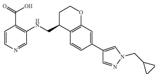
3-({[(4S)-7-[1-(cyclopropylmethyl)-1H-pyrazol-4-yl]-3,4-dihydro-2H-1-benzopyran-4-yl]methyl}amino)pyridine-4-carboxylic acid
