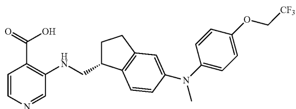
3-({[(1R)-5-{methyl[4-(2,2,2-trifluoroethoxy)phenyl]amino}-2,3-dihydro-1H-inden-1-yl]methyl}amino)pyridine-4-carboxylic acid
