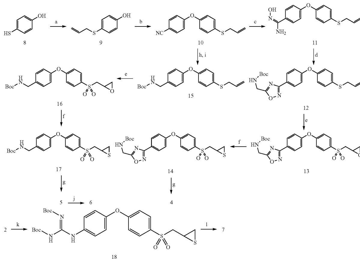
Scheme 1. Syntheses of the inhibitors 4, 5, 6 and 7 a .
